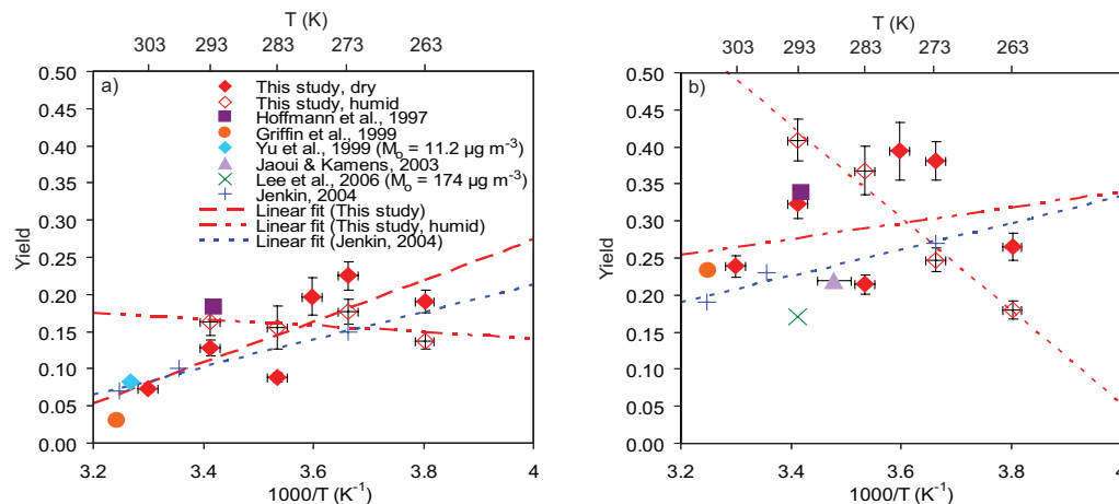
Fig. 6. Secondary organic aerosol yield ( Y ) plotted against inverse temperature ( 1000/T ): (a) M_0 = 10 \mu\text{g m}^{-3} ; (b) : M_0 = 250 \mu\text{g m}^{-3} . The symbols represent measurement or two-product model results of different studies. The error bars of the yield represent the standard deviations of 4–24 replicate measurements from our experiments with M_0 close to 10 \mu\text{g m}^{-3} or 250 \mu\text{g m}^{-3} respectively. The error bars of the temperature represent the confidence interval of the thermo sensors applied in our study and the range of temperatures reported in other studies. Lines are linear fits.
