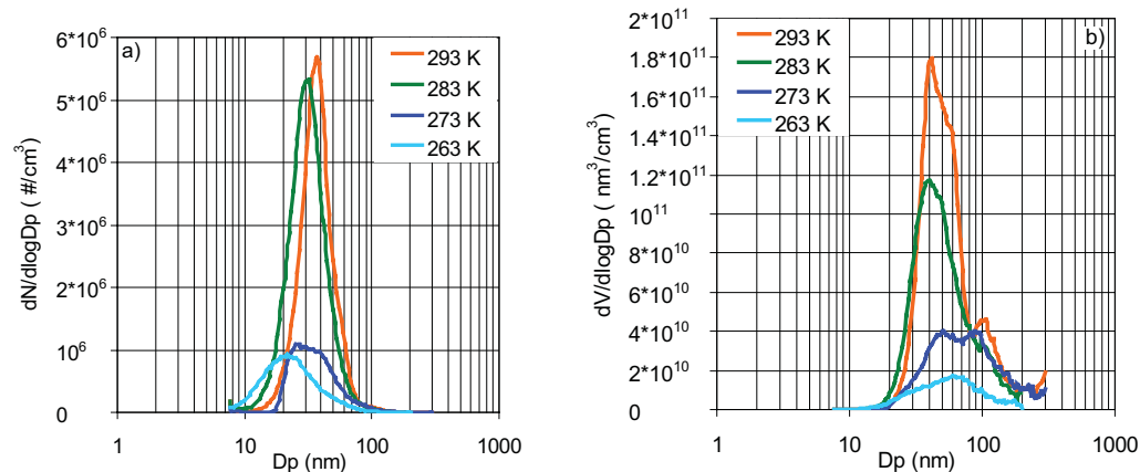
Fig. 3. Particle number (a) and volume (b) size distributions from humid experiments with [\beta\text{-pinene}]_0 = 0.97 \text{ ppmv}–1.76 \text{ ppmv} and [\text{O}_3]_0 \approx 1.25 \text{ ppmv} (except for 263 K: [\text{O}_3]_0 = 0.9 \text{ ppmv} ) at different temperatures (263 K–293 K).
