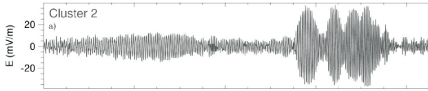
Fig. 1. Modulated structures, related to “chorus” (EM) emission in the magnetosphere (CLUSTER satellite data; reprinted from Santolik, 2003).
