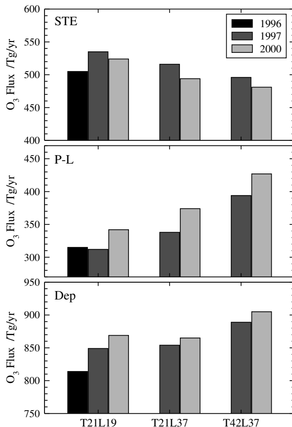
Fig. 4. Effects of meteorology and model resolution on the annual flux of O_3 through stratosphere-troposphere exchange (STE), net chemistry (P-L) and surface deposition (Dep).
