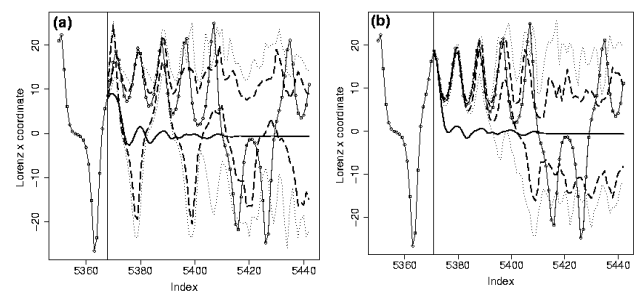
Fig. 3. Same as Fig. 2 but for Lorenz x coordinate, blind prediction starts from (a) index 5368, and (b) index 5371.
