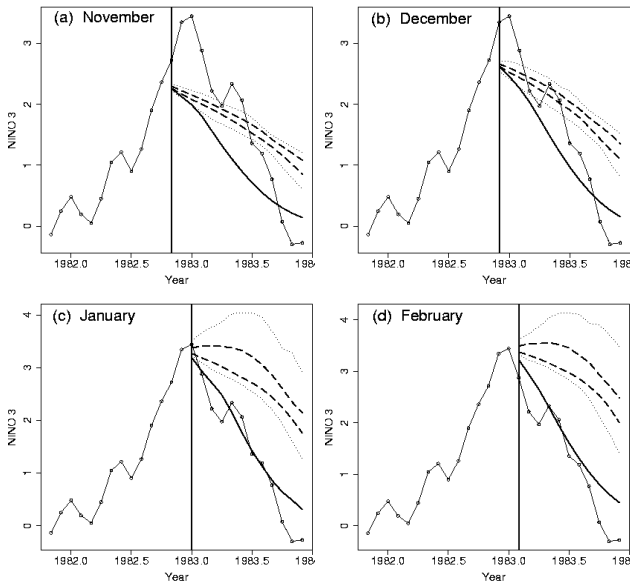
Fig. 6. Same as Fig. 2 but for the NINO3 index. Blind forecast of 1982–1983 El Niño event issued from different starting points (a) November 1982, (b) December 1982, (c) January 1983, and (d) February 1983.
