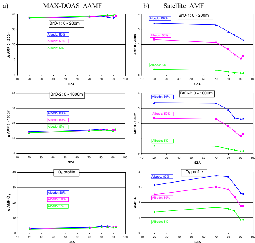
Fig. 2. \Delta AMFs for MAX-DOAS observations at 1^\circ elevation angle (left) and AMFs for satellite observations (right) for various values of the surface albedo and different height profiles (see Fig. 1). While the sensitivity of the satellite observations strongly depends on the surface albedo and the solar zenith angle, the \Delta AMFs for the MAX-DOAS observations are almost not affected. For the surface near profile the sensitivity of the MAX-DOAS observations is about one order of magnitude larger compared to the satellite observations.
