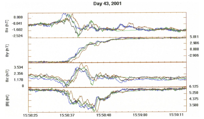
Fig. 15. A MD detected by all four CLUSTER spacecraft. The MD is at the edge of a phase-steepened Alfvén wave.
