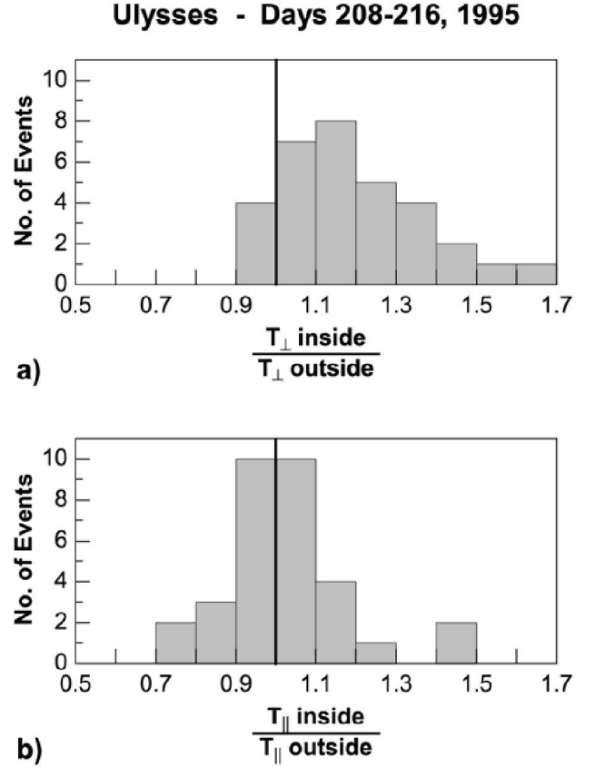
Fig. 8. The ratios of the inside to outside (the MD) parallel and perpendicular proton temperatures. The proton perpendicular temperatures are higher inside the MD than outside the structure.
