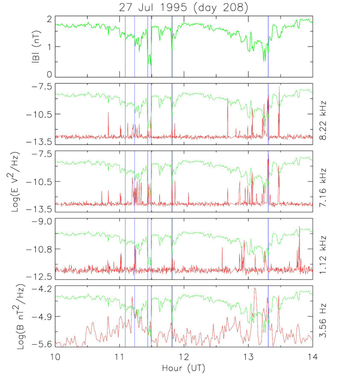
Fig. 10. The relationship between electrostatic noise between 1.12 and 8.22 kHz and MHs/MDs.
