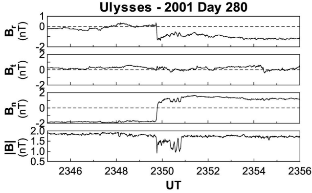
Fig. 9. Mirror mode structures within a MD. Several oscillations can be noted from 23:50:20 to 23:50:50 UT.
