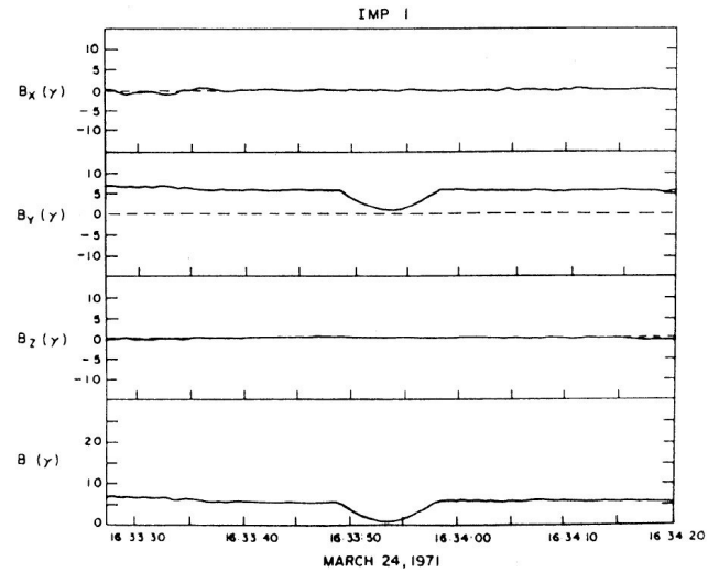
Fig. 2. An example of a magnetic hole (MH) at 1 AU. Taken from Turner et al. (1977).
