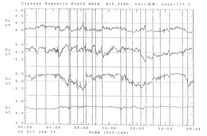
Fig. 4. Interplanetary directional discontinuities (vertical lines).
