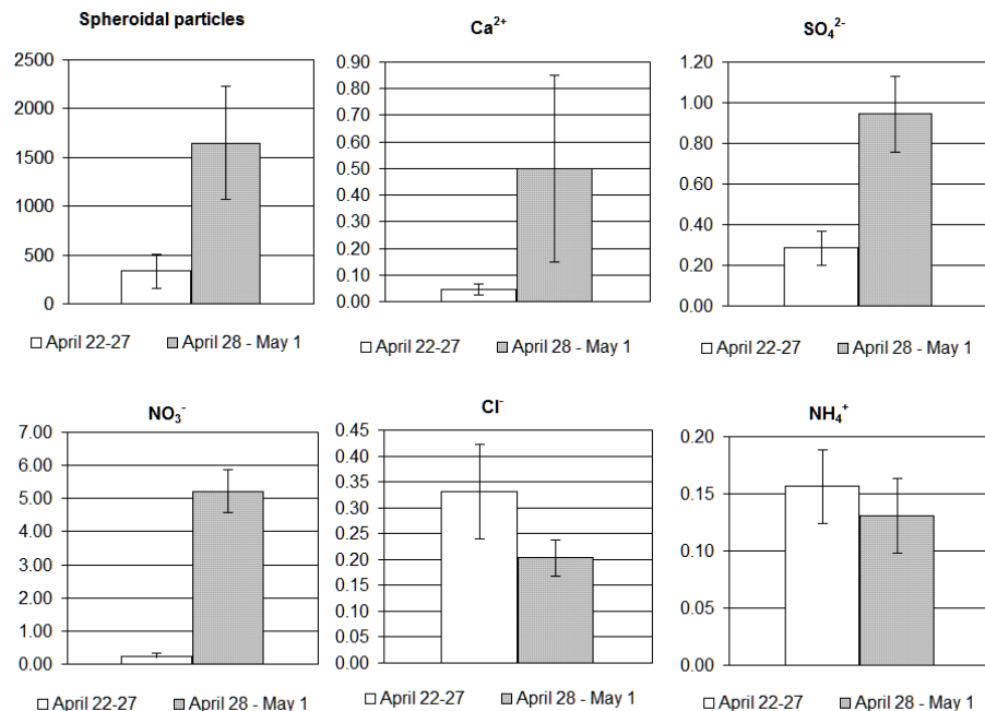
Fig. 5. Average deposition fluxes with error bars of inorganic compounds and spheroidal particles of two sampling periods during the LAPBIAT measurement campaign, in \text{# m}^{-2} per day for spheroidal particles and \text{mg m}^{-2} per day for other species. The fluxes are based on snow samples that were collected from several locations close to SMEAR I station.
