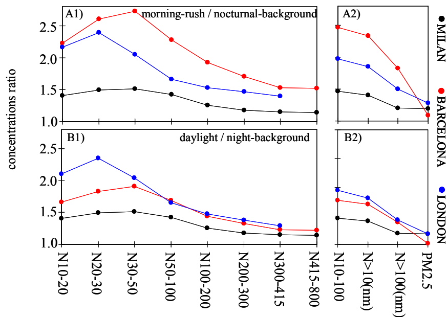
Fig. 4. “Morning rush hours (06:00–08:00) to nocturnal-background (02:00–05:00)” and “daylight (06:00–18:00) to night-background (02:00–05:00)” ratios of the aerosol PM 2.5 mass and number concentration in several size ranges during working days of the 1-year study period.
