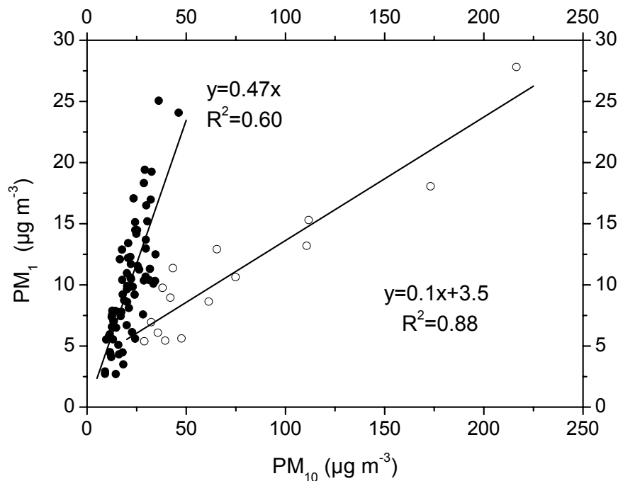
Fig. 2. PM 1 versus PM 10 for the sampling period. All fractions are referred to measurements from the SDI. Regression lines are calculated and data obviously influenced by dust are shown as open circles and separate regression is performed.
