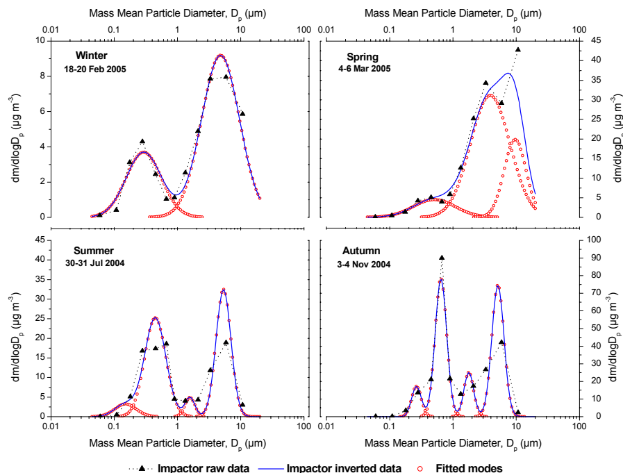
Fig. 5. Typical examples of mass distributions per season. The plots include raw gravimetric stage mass concentrations (impactor raw data) and continuous distributions after applying the collection efficiency curves of the impactor (inversion – impactor inverted data). Finally, a number of lognormal distributions are fitted to separate between the different modes of each distribution.
