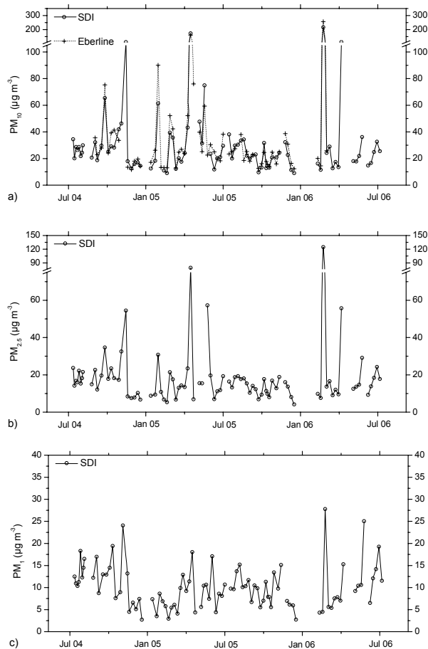
Fig. 1. \text{PM}_{10} , \text{PM}_{2.5} and \text{PM}_1 fractions measured at Finokalia for the period July 2004–July 2006 using the SDI and the Eberline FH 62 I-R Particulate Monitor.
