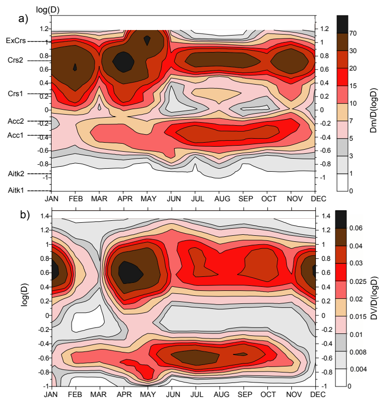
Fig. 8. Annual variation of the particle size distribution derived from (a) the SDI mass size distributions measured at ground surface and (b) the AERONET columnar size volume-distributions. The ordinates correspond to the logarithm of the mean mode diameters. Aerodynamic and physical diameters are used for the SDI and the AERONET, respectively. The color scale represents integrated (a) mass and (b) volume of particles per interval of \log(D) .
