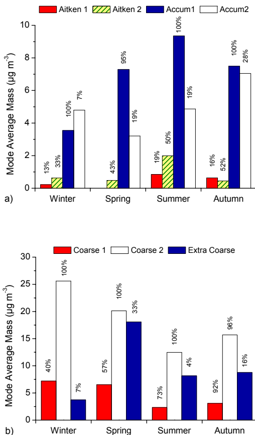
Fig. 7. Seasonal variability of the average mass of each mass mode for the period July 2004–July 2006. The modes are presented separately for the fine (a) and the coarse (b) part of the masses. Numbers on the top of the columns indicate the frequency of occurrence of that mode into the measured distributions per season.
