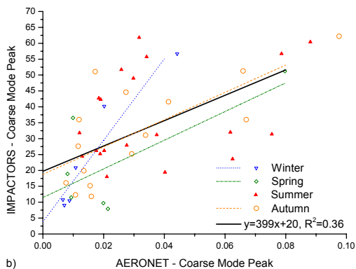
Fig. 10. Scatterplot between the peak values from the SDI and the AERONET distributions. Peaks are coupled for the fine (a) and the coarse modes (b) and are presented with different symbols for each season. Linear fittings are performed for each season and are shown together with an overall regression line when strong relationship is found.
