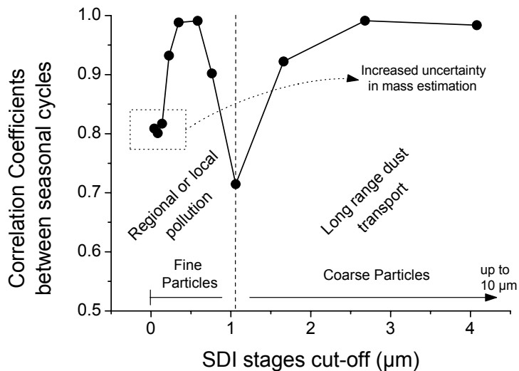
Fig. 4. Correlation coefficients between the seasonal cycles from the adjacent stages of the SDI. The coefficient is attributed to the stage with the lower cut-off.
