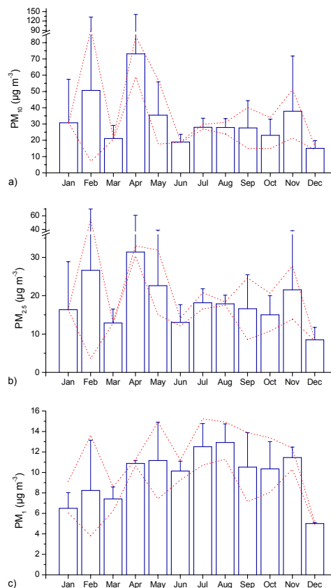
Fig. 3. Seasonal cycles of (a) \text{PM}_{10} , (b) \text{PM}_{2.5} and (c) \text{PM}_1 fractions at Finokalia derived from the SDI measurements during the period July 2004–July 2006. The error bars correspond to the standard deviation of all samples per month during the whole period while the dotted lines correspond to the standard deviation after extracting monthly averages.
