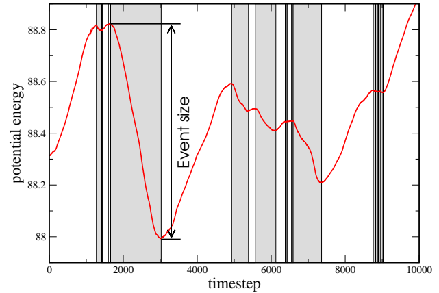
Fig. 11. Original potential energy time series with picked events (in gray) and calculation of event size illustrated.
