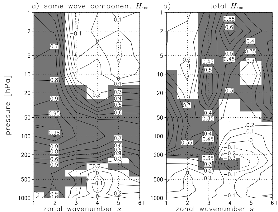
Fig. 3. Correlation coefficients of a) the zonal wave- s component of H_{100} , and b) H_{100} , with the zonal wave- s component of \langle v * T^* \rangle_{NH} . Correlation coefficients are calculated over 1958–2002, and the areas with > 95% confidence levels are shaded.
