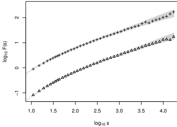
Fig. 6. DFA1 (+) and DFA2 ( \Delta ) fluctuation function of Prague daily air temperature data calculated for approximately 50 points per order of magnitude. Only every 4th point is shown to enhanced clarity. The shadows mark the 1.96\sigma confidence regions derived from 1000 runs of the AR model.
