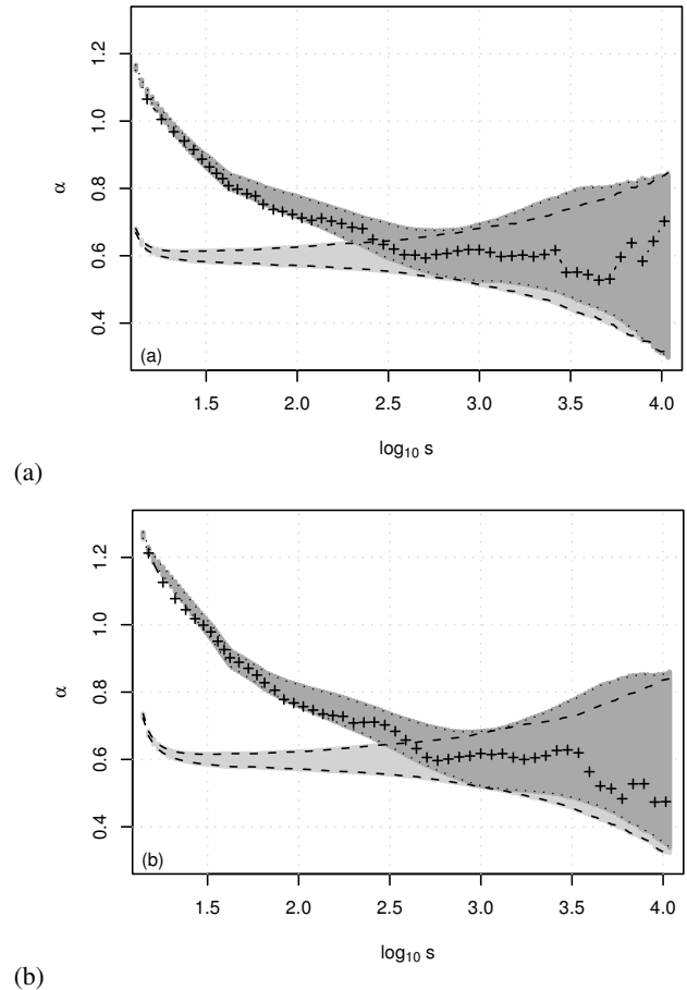
Fig. 7. Local slopes of the fluctuation functions plotted in Fig. 6 for (a) DFA1 and (b) DFA 2 of the Prague daily temperature data. The dotted lines border the 1.96\sigma confidence regions of the short-range correlated model Eq. (10) (dark shadow), the dashed lines those of the long-memory model with \alpha=0.6 (light shadow).
