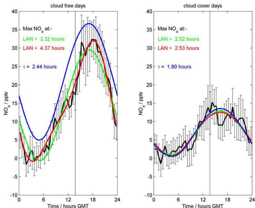
Fig. 2. Daily averaged time series of NO x (No + NO 2 ) for the same data as in Fig. 1, with the cloud free data on the left and the cloud cover data on the right. Overlaid on each plot are three functions fitted to the binned data by least squares. In green and red are harmonic functions; the green function uses a single harmonic as per Eq. (6), the red function has first and second harmonics as per Eq. (7). For the cloud free days, the red curve is a significantly better fit, implying an asymmetry to the NO x time series. The harmonic functions for the cloud cover data are equivalent. The blue curves show diffusion model fits, where \tau has been tuned to give the same post-LAN maximum as the single harmonic function. For the cloud free data there is a significant mean discrepancy between the diffusion model and the data, whilst for the cloud cover days, this offset is absent, implying some real effect, and not an artefact of the instrument.
