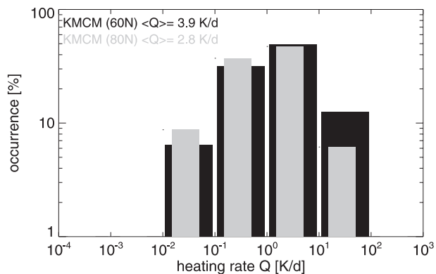
Fig. 6. Histograms of the energy dissipation rates (here shown as equivalent heating rates) at 60° N and 80° N from the model study of Becker and Fritts (2006) for permanent July conditions. Mean values are indicated in the insert.
