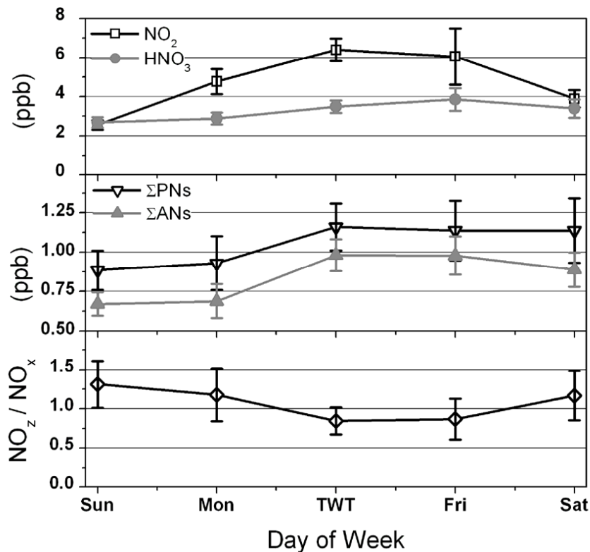
Fig. 13. Speciated \text{NO}_{y_i} observations from Granite Bay all made between 10:00 and 18:00 during the summer of 2001. The top panel shows measurements \text{NO}_2 and \text{HNO}_3 . The middle panel shows measurements of sum peroxy nitrates and sum alkyl nitrates. In the bottom panel, the diamonds correspond to the left axis and show the ratio of \text{NO}_z to \text{NO}_x in the airmass ( \text{NO}_z \equiv \Sigma\text{PNs} + \Sigma\text{ANs} + \text{HNO}_3 ). Error bars are twice the standard deviation of the mean.
