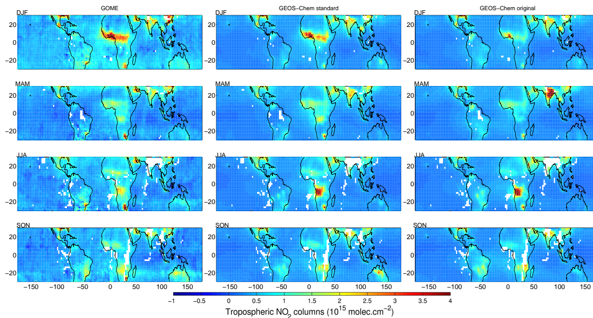
Fig. 6. Seasonal averaged tropospheric \text{NO}_2 columns ( 10^{15} \text{ molec cm}^{-2} ) during the year 2000. The left panels are for GOME, the middle for GEOS-Chem standard and the right for GEOS-Chem original. White areas indicate regions with persistent clouds.
