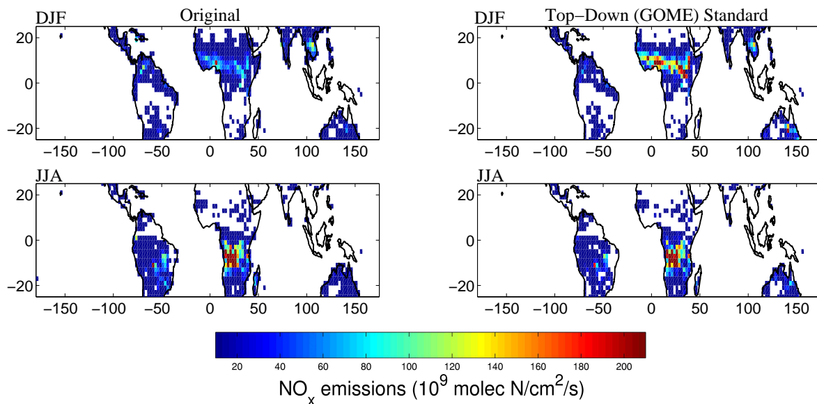
Fig. 2. Seasonal biomass burning emissions ( 10^9 \text{ molec N cm}^{-2} \text{ s}^{-1} ) for December-February (DJF) and June-August (JJA). The left panels represent emissions used in the original simulation. The right panels represent top-down emissions determined from GOME observations of tropospheric \text{NO}_2 columns.
