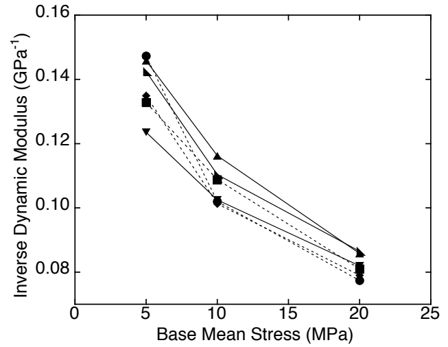
Fig. 11. K_{\text{dyn}}^{-1} and G_{\text{dyn}}^{-1} for \tau = 1 \text{ MPa} . The squares, circles, and diamonds connected by dotted lines are K_{\text{dyn}}^{-1} , for \theta , \tau , and \mu constant respectively. The triangles connected by solid lines are G_{\text{dyn}}^{-1} : triangles pointing up for \theta constant, right triangles for \mu constant, and triangles pointing down for \sigma constant.
