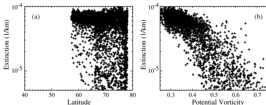
Fig. 2. This figure depicts a comparison of the distribution of 1020-nm aerosol extinction coefficient from SAGE III in January through March of 2003 through 2005 at 20 km. Frame (a) shows the distribution as a function of latitude while frame (b) shows the distribution as a function of potential vorticity in units of \text{km}^2\text{s}^{-1}\text{kg}^{-1} times 10^4 .
