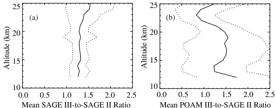
Fig. 14. (a) Mean profile of the ratio of SAGE III 449 to 1020-nm aerosol extinction ratio and the SAGE II 452 nm to 1020-nm aerosol extinction ratio for the winters of 2003 through 2005. The solid line is the mean while the dotted line is the 1-sigma confidence limits. (b) Same as frame (a) except for POAM III 442 nm to 1018 nm aerosol extinction ratio and the SAGE II 452 to 1020-nm aerosol extinction ratio.
