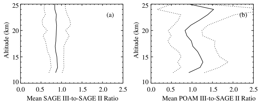
Fig. 9. (a) Mean profile of the ratio of SAGE III and SAGE II 1020-nm aerosol extinction coefficients for the winters of 2003 through 2005. The solid line is the mean while the dotted line is the 1-sigma confidence limits. (b) Same as frame (a) except for POAM III and SAGE II.
