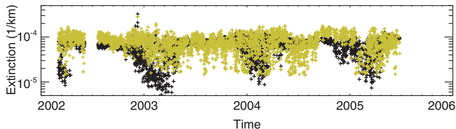
Fig. 1. This figure shows the 18-km, 1020-nm aerosol extinction coefficient measured by SAGE III (black) and POAM III (gold) in the Northern Hemisphere. Note that this figure shows all observations by each instrument with no matching requirement.
