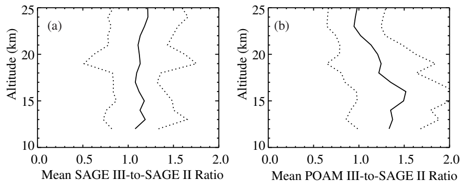
Fig. 12. (a) Mean profile of the ratio of SAGE III 449 nm and SAGE II 452-nm aerosol extinction coefficients for the winters of 2003 through 2005. The solid line is the mean while the dotted line is the 1-sigma confidence limits. (b) Same as frame (a) except for POAM III 442 nm and SAGE II 452-nm aerosol extinction coefficient.
