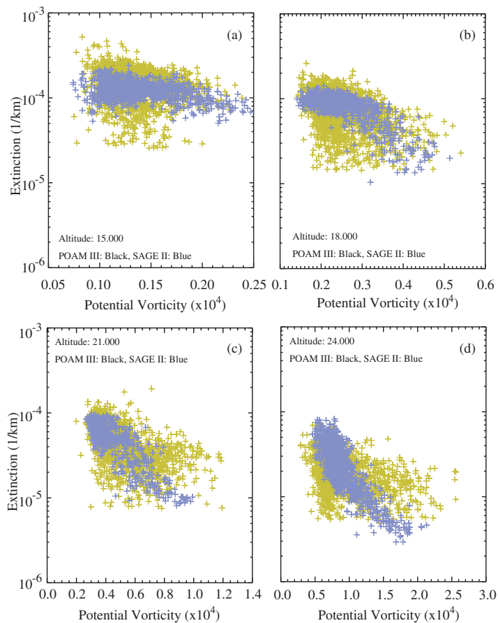
Fig. 6. This figure shows the distribution of 1020-nm aerosol extinction coefficient measured by POAM III (gold) and SAGE II (blue) at 15 (a), 18 (b), 21 (c), and 24 km (d) for January through March of 2003 through 2005. The plots show all data without any matching requirements.
