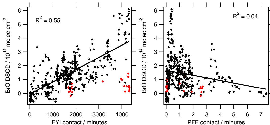
Fig. 3. Correlation plots of BrO versus first-year sea-ice contact (left) and potential frost flowers contact (right). Data colored in red occurred when ozone <1 ppbv and were ignored from the correlation analysis.
