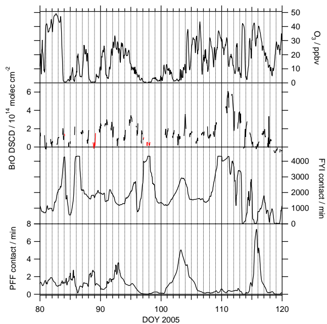
Fig. 2. Ozone, Bromine monoxide (BrO), first-year sea-ice contact (FYI), and potential frost flowers contact (PFF) timeseries in the period DOY 80–120. BrO data colored red occurred when ozone < 1 ppbv.
