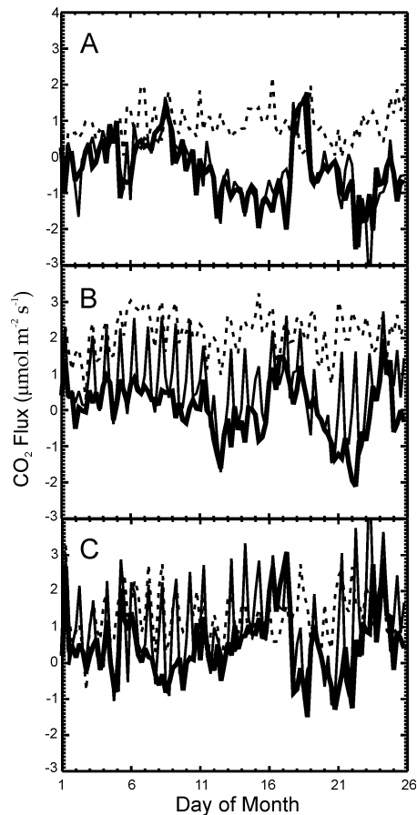
Fig. 4. (a) The evenly-weighted footprint-average NEE predicted by SiB2 for the measurements shown in Fig. 1. Line types correspond to those used in Fig. 1; (b) The footprint-mean NEE calculated using the first term on the right-hand side of (11) or (5); (c) The value of the covariance term.
