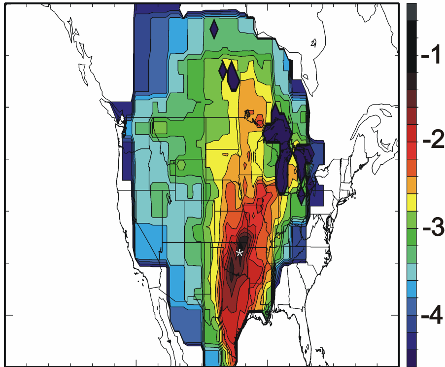
Fig. 1. Logarithm of the average footprint ( \text{ppm } (\mu\text{mol m}^{-2} \text{s}^{-1})^{-1} ) for July measurements at 500 m. Approximate location of ARM-CART SGP denoted by star. The Great Lakes and other water bodies were given a value of zero.
