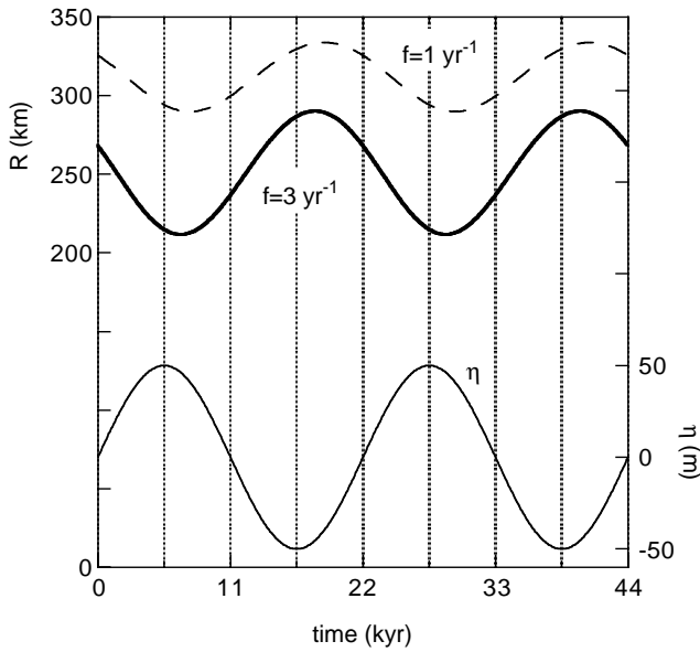
Fig. 7. Response of a marine ice sheet to periodic forcing of sea level ( \eta ), for two values of the grounding-line flux parameter f . Model parameters: s = 0.001 , d_0 = 150 m, h_E = 150 m, A = 1 m/yr, C_R = 500 km.
