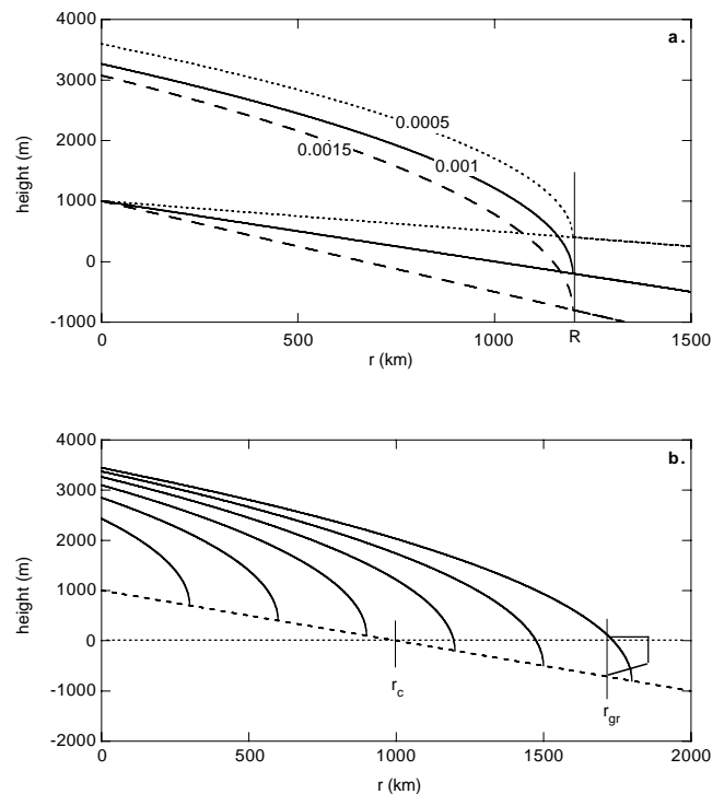
Fig. 1. (a) Geometry of the model ice-sheet for three values of the slope of the undisturbed bed (labels). Note that the actual bed, which is depressed by the ice load, is not shown. (b) Geometry for different values of the ice-sheet radius. At r = r_c the terminus of the ice-sheet enters the sea. The undisturbed bed slope is 0.001. Other parameter values are: d_0 = 1000 m, \mu_0 = 8 m 1/2 , c = 2 \cdot 10^6 m 1/2 .
