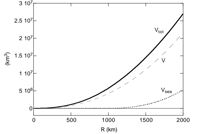
Fig. 2. Total ice-sheet volume ( V_{tot} ) as a function of the ice-sheet radius R . Volume in the case of no bed response ( V ) and the amount of displaced sea water ( V_{sea} ) are also shown. Model parameters as for Fig. 1.
