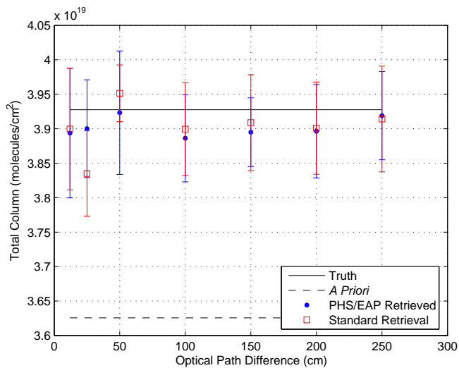
Fig. 7. Simulated retrievals of CH 4 columns, assuming SNR=250, as a function of OPD.
