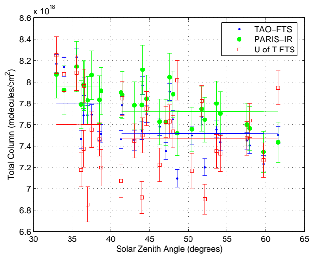
Fig. 14. As in Fig. 13, but for O_3 in the 2775\text{ cm}^{-1} microwindow.
