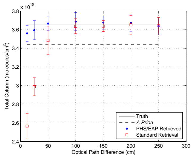
Fig. 5. Simulated retrievals of HCl columns, assuming SNR=250, as a function of OPD.
