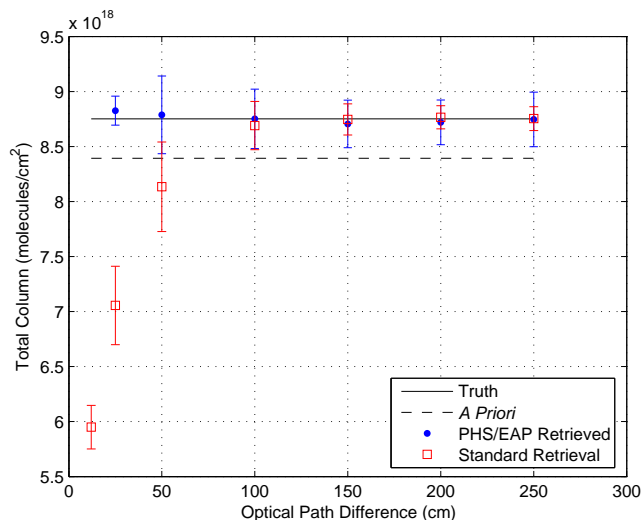
Fig. 4. Simulated retrievals of ozone columns in the 2775\text{ cm}^{-1} microwindow, assuming \text{SNR}=250 , as a function of OPD. The small error bars on the PHS/EAP retrieval for 25 cm OPD are due to the small number of retrievals that converged for this OPD. The error bars are, as a consequence, artificially small.
