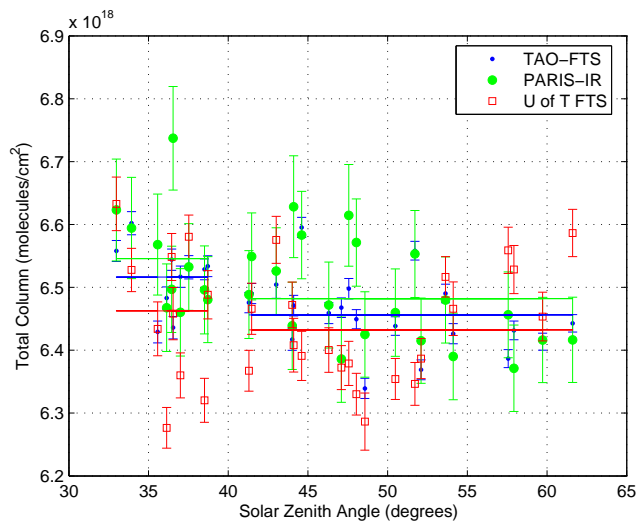
Fig. 16. As in Fig. 13, but for N_2O .
