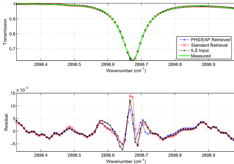
Fig. 12. \text{CH}_4 spectral fits for the U of T FTS (upper panel), and the corresponding residuals (lower panel).
