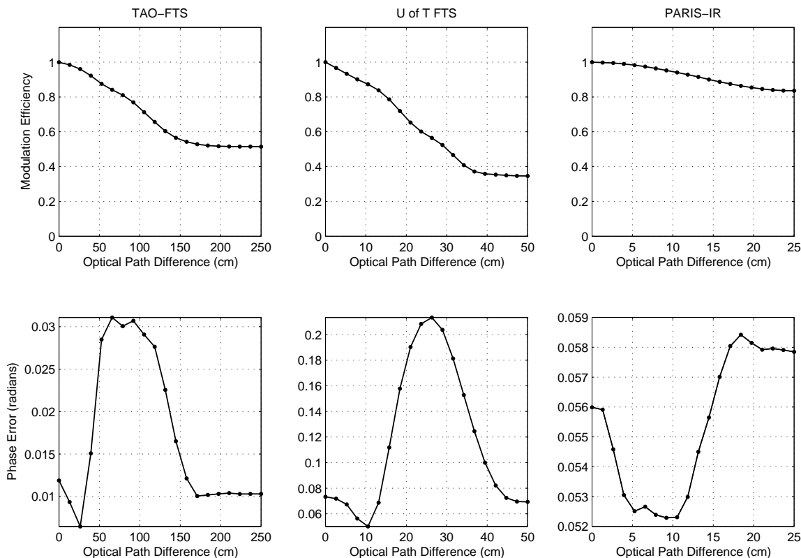
Fig. 1. Typical modulation efficiency and phase error for all three instruments. These are computed from gas cell measurements using the LINEFIT software (Hase et al., 1999). The top panels contain the modulation efficiency and the lower panels contain the phase error. The left-most panels show unapodized TAO-FTS data, recorded in August, 2005. The central panels show U of T FTS data, apodized with a triangular filter and recorded in September, 2005. The right-most panels show unapodized PARIS-IR data, recorded in August, 2005.
