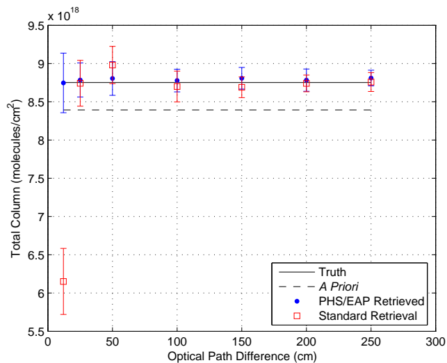
Fig. 3. Simulated retrievals of ozone columns in the 3040\text{ cm}^{-1} microwindow, assuming \text{SNR}=250 , as a function of OPD.
