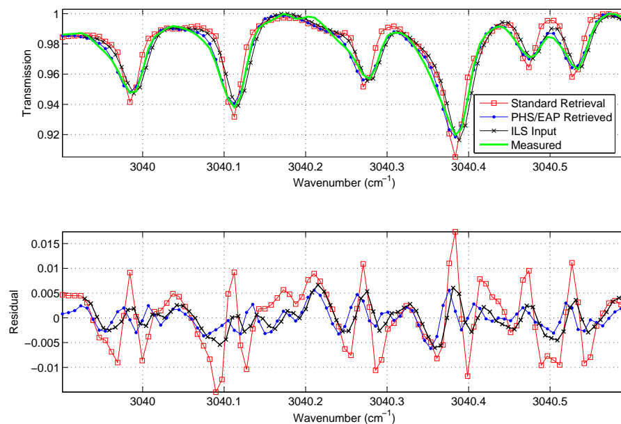
Fig. 9. O 3 (3040) spectral fits for the U of T FTS (upper panel), and the residuals between the measured retrieval and the spectral fits (lower panel).
