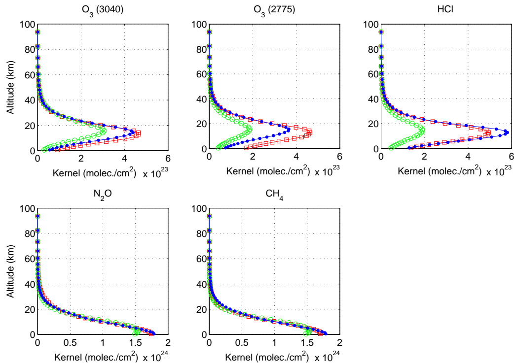
Fig. 18. Density-weighted column averaging kernels for the three instruments: TAO (blue dots), U of T FTs (red squares) and PARIS-IR (green circles), illustrating the sensitivity of the retrieved column at each altitude.
