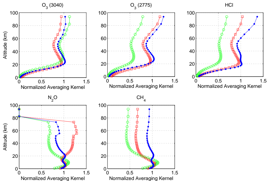
Fig. 19. Normalized column averaging kernels. These panels show the normalized column averaging kernels for for the three instruments: TAO (blue dots), U of T FTS (red squares) and the PARIS-IR (green circles).
