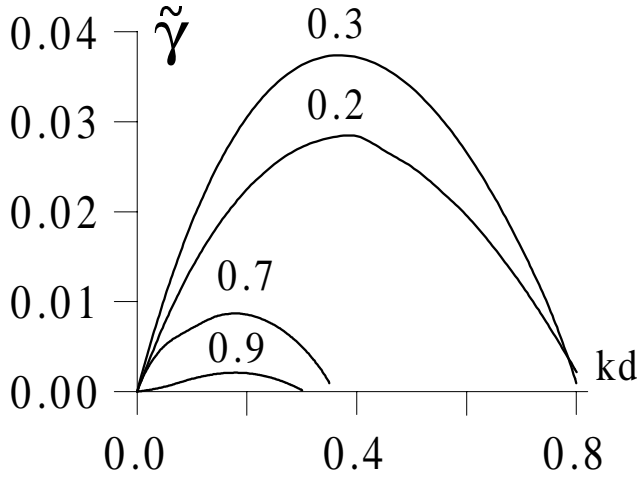
Fig. 5. Influence of \cos \phi on the dependence of the growth rate \tilde{\gamma}(kd) for the magnetic field aligned with the flow \mathbf{v}_0 , or \mathbf{B}_0 = \mathbf{B}_{0||} when M = 2 , \beta = 1.5 , M_{ms} = 1.49 , and \rho = const . The value of \cos \phi is shown above the curves.
