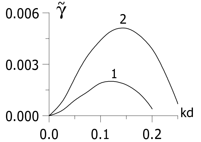
Fig. 2. Influence of the magnetic component \mathbf{B}_{0\perp} (perpendicular to the flow velocity \mathbf{v}_0 ) on the dependence of the growth rate \tilde{\gamma}(kd) of supersonic longitudinal disturbances ( \mathbf{k} parallel to the flow velocity \mathbf{v}_0 , or \mathbf{k} = \mathbf{k}_{\parallel} ) when M = 2 . Curves 1 and 2 correspond to the following values of the parameter \beta : \beta = 100 ( M_{ms} \approx M = 2 ) and \beta = 2 ( M_{ms} = 1.58 ).
