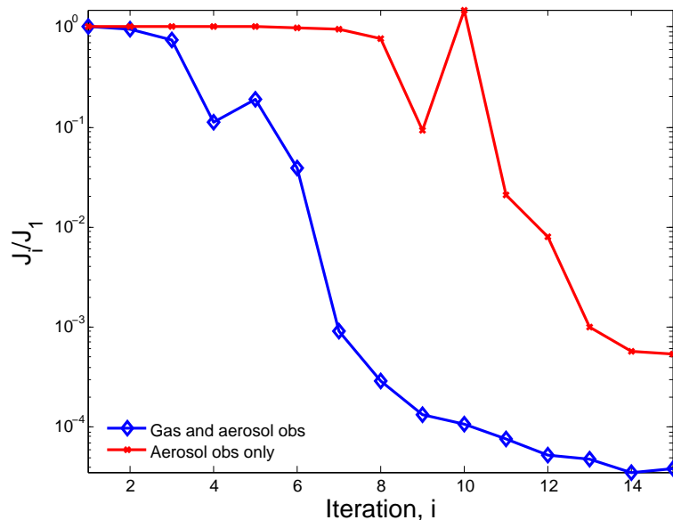
Fig. 10. Cost function reduction for tests DA2. A uniform perturbation is applied to emission inventories of anthropogenic \text{NH}_3 . Complete daily measurements of (red-crosses) ammonium aerosol and (blue-diamonds) ammonium aerosol and gas-phase \text{O}_x are utilized for the data assimilation during a week-long simulation.
