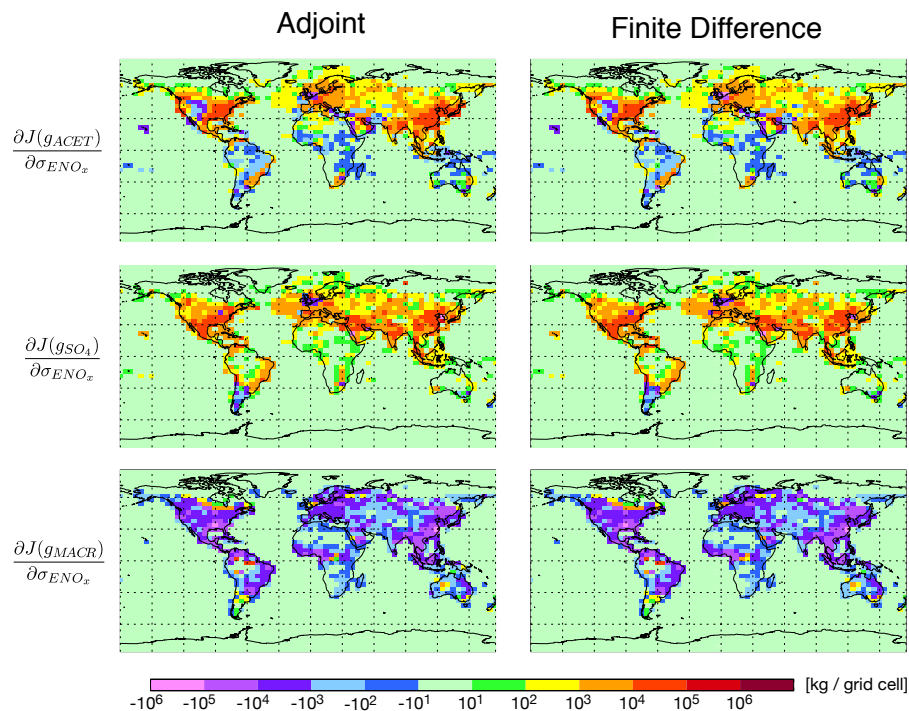
Fig. 2. Chemistry adjoint validation. Full chemistry (only) simulation for 1 week. In the left column are the gradients of the masses of acetone (ACET), sulfate aerosol (SO 4 ), and methacrolein (MACR) at the surface with respect to anthropogenic emissions of NO x . In the right column are the same quantities calculated using the finite difference method.
