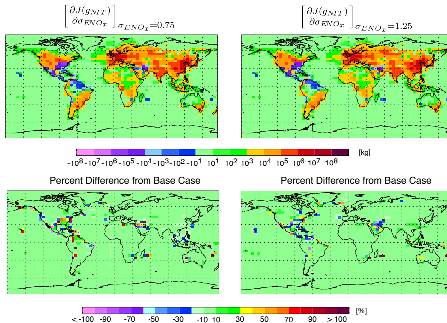
Fig. 8. Sensitivities of nitrate aerosol to emissions of anthropogenic \text{NO}_x when the emission inventories are scaled by factors of 0.75 and 1.25, and the percent difference between these sensitivities and those calculated with the base case ( \sigma_{\text{ENO}_x} = 1.0 ), shown in Fig. 7.
