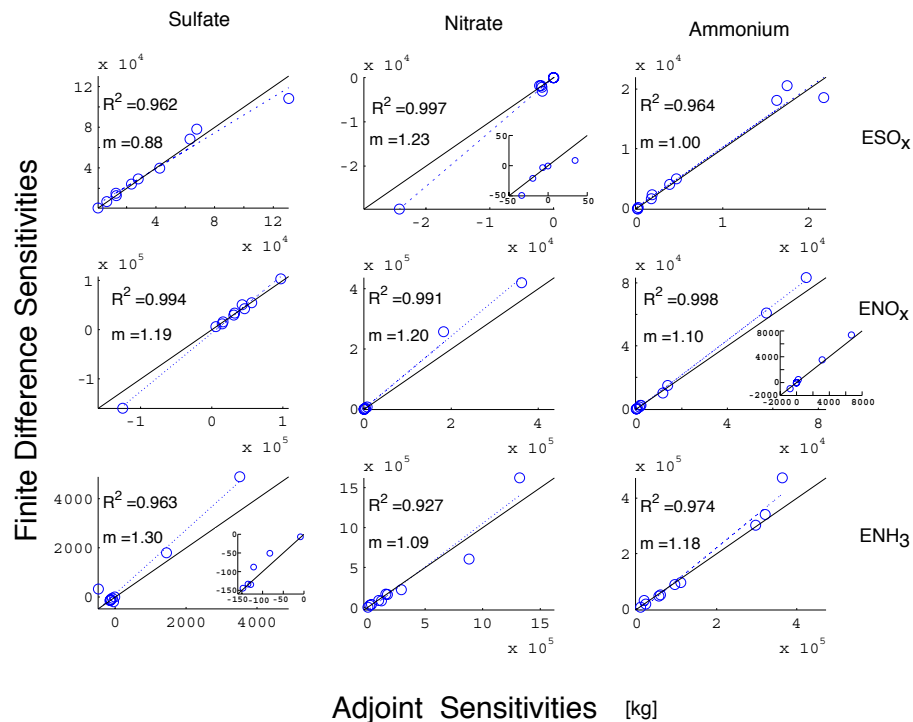
Fig. 4. Overall accuracy. Comparison of sensitivities of global aerosol burdens to anthropogenic precursor emissions calculated using the adjoint method vs. the finite difference method. A few of the plots contain insets with magnified views of a cluster of points.
