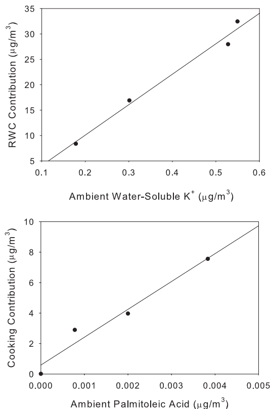
Fig. 1. Comparison of average residential wood combustion (RWC) and cooking contributions and average ambient water-soluble potassium ( K^+ ) and palmitoleic acid concentrations during four CRPAQS winter intensive periods at the Fresno Supersite in California. The values represent averages from the four sample periods during the winter intensive study (00:00–05:00, 05:00–10:00, 10:00–16:00, and 16:00–24:00 PST).
