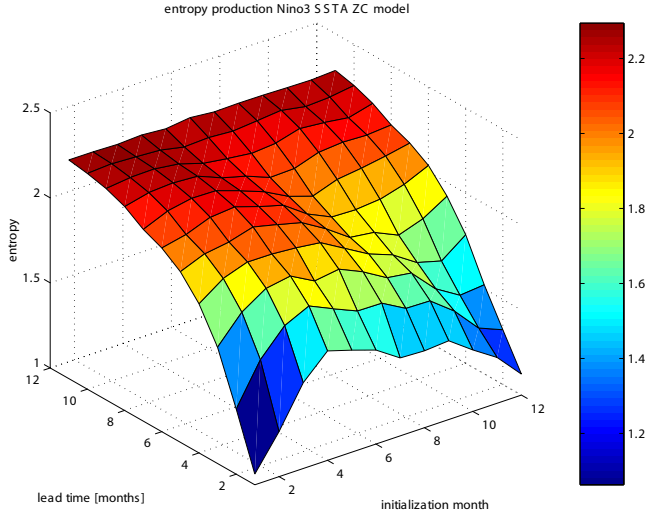
Fig. 2. Seasonal dependence of the entropy production: Entropy as a function of lead time and of the initialization month.
