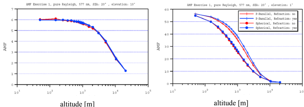
Fig. 11. Box-AMFs calculated by the Japanese model for an elevation angle of 10° (left) and 1° (right) for a pure Rayleigh atmosphere (solar zenith angle: 20°, relative azimuth angle: 0°, wavelength: 577 nm). If the Earth's sphericity is not taken into account, large errors can occur (up to a factor of two). In contrast, refraction has only a relatively small influence on the box-AMFs.
