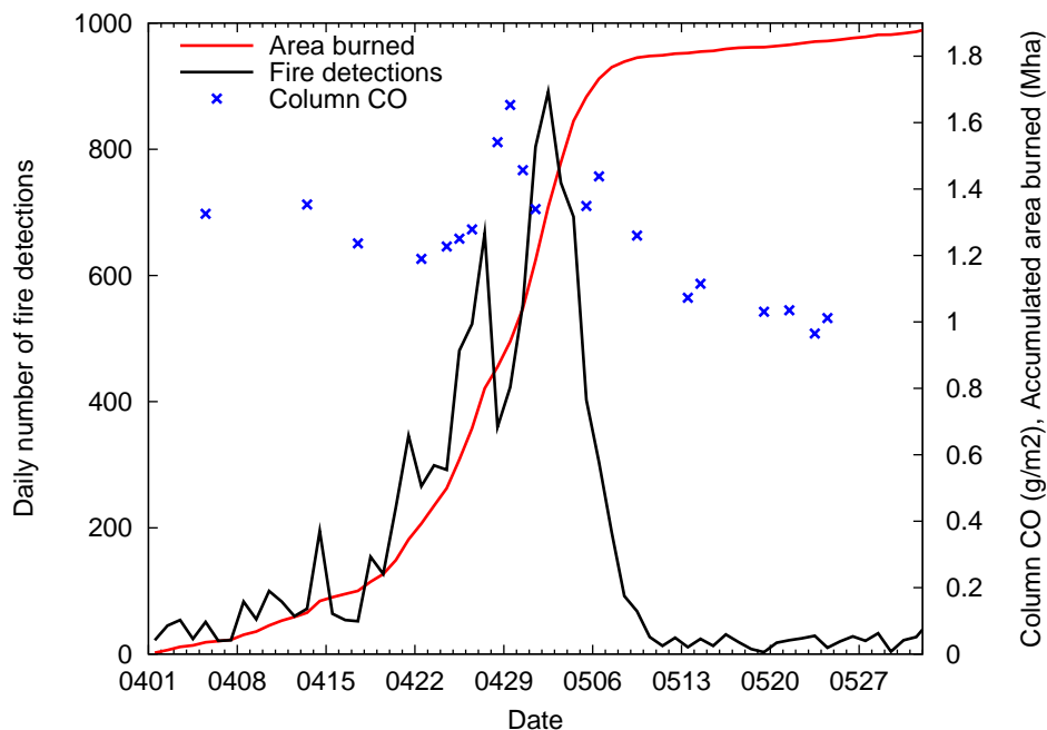
Fig. 3. Time series of daily number of MODIS fire detections in the region north of 40^{\circ}\text{N} and between 20^{\circ}\text{E} and 60^{\circ}\text{E} (black line) and estimated area burned in this region, accumulated from 1 April 2006 and assuming that 180 ha burned per detected fire (red line). Also shown are measurements of total column CO taken at Zvenigorod (blue symbols).
