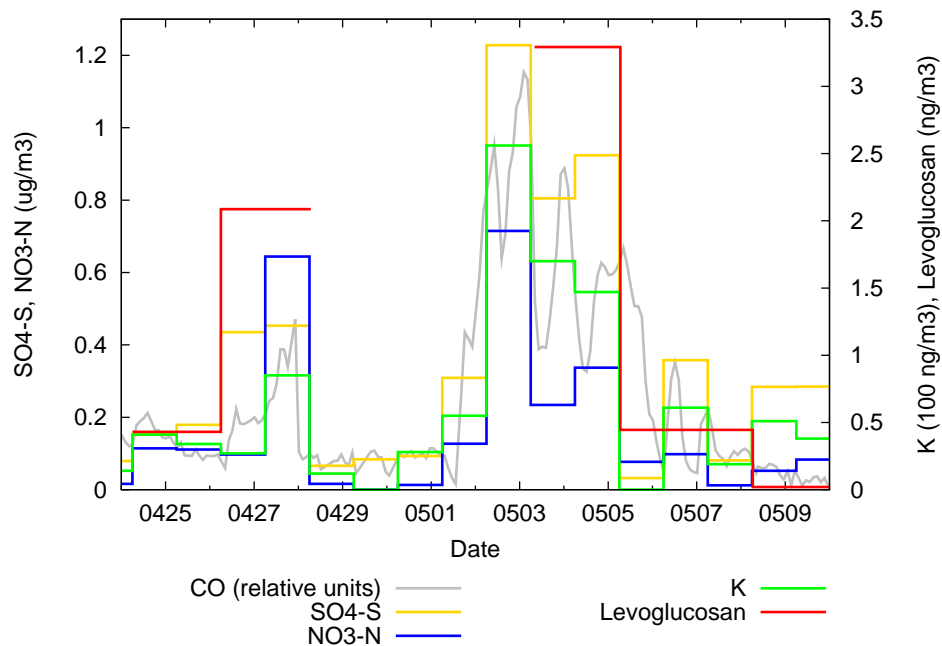
Fig. 21. Time series of CO, and \text{NO}_3^- -N, \text{SO}_4^{2-} -S and \text{K}^+ from daily, and levoglucosan from irregular filter samples taken at Zeppelin.
