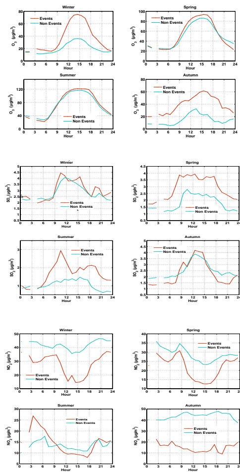
Fig. 13. Hourly averages of O 3 , SO 2 and NO 2 ( \mu\text{g}/\text{cm}^3 ) respectively over all seasons on event and non-event days.
