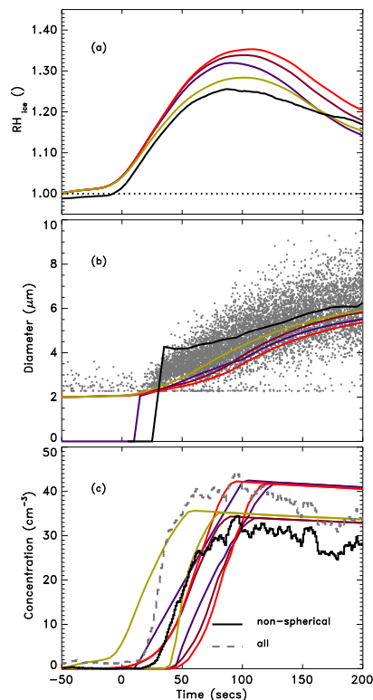
Fig. 10. Expansion 44 (Saharan dust SD2) with initial chamber temperature -60^{\circ}C . On each panel, the black line represents the observations (for the diameter, it is the median of all particles with a diameter greater than 4 \mu m ). The purple line is for the model with the ice nucleation modes parametrised as before, by just inserting ice particles to match the SID observations. The brown and red lines are for models which assume deposition nucleation following Meyers et al. (1992) and the mustard line using Eq. (6). On panel (c), the left-most line is the concentration of all ice crystals and the right-most line only ice crystals greater than 3 \mu m .
