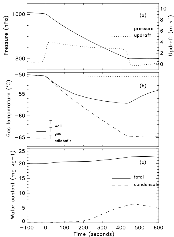
Fig. 1. An example chamber expansion (experiment 28) showing the chamber pressure change (a) , and the resultant cooling (b) . The effect of the wall vapour flux is shown in panel (c) . The time axis is plotted in seconds relative to the start of pumping. There is also a decrease in chamber pressure before the actual expansion starts due to the particle probes sampling the chamber gas.
