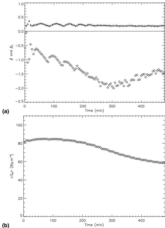
Fig. 11. Time evolution of (a) the ratios of the entrainment flux to the surface flux for potential temperature (crosses) and ^{222}\text{Rn} (diamonds), and (b) ^{222}\text{Rn} mixed-layer concentration \langle S_0 \rangle .
