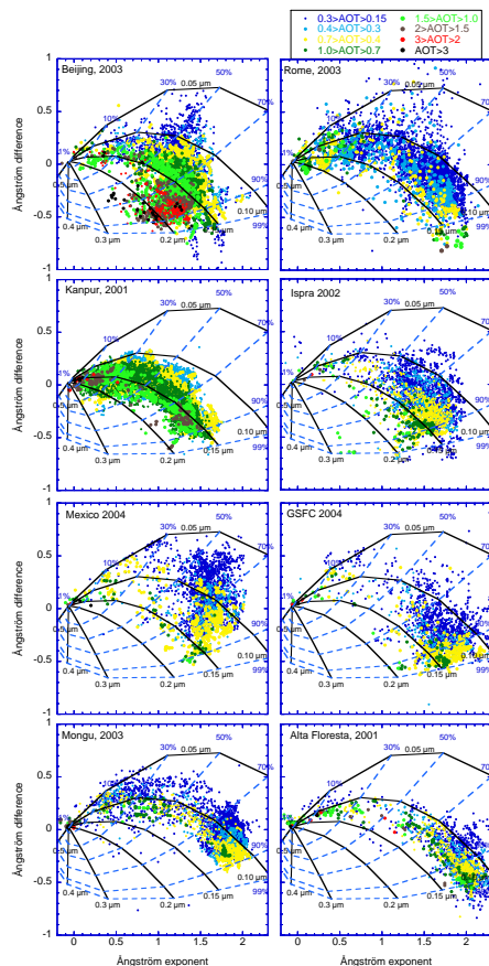
Fig. 3. Angstrom exponent difference, \delta\alpha = \alpha(440, 675) - \alpha(675, 870) , as a function of the 440–870 nm Angström exponent and AOT (color code) for eight AERONET stations (from top): Beijing (China), Rome (Italy), Kanpur (India), Ispra (Italy), Mexico City (Mexico), GSFC (USA), Mongu (Zambia) and Alta Floresta (Brasil). Only cloud-screened data with \text{AOT} > 0.15 were used.
