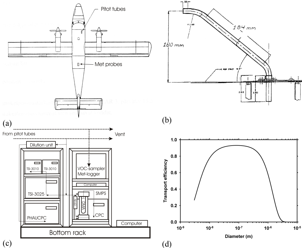
Fig. 1. (a) Schematic of the GTK Twinn Otter and location of Pitot and met-probe tubes; (b) schematic of aerosol Pitot inlet tube; (c) schematic of aerosol instrumentation rack; (d) calculated aerosol losses of air speed of 0.75 \times 55 \text{ m s}^{-1} .
