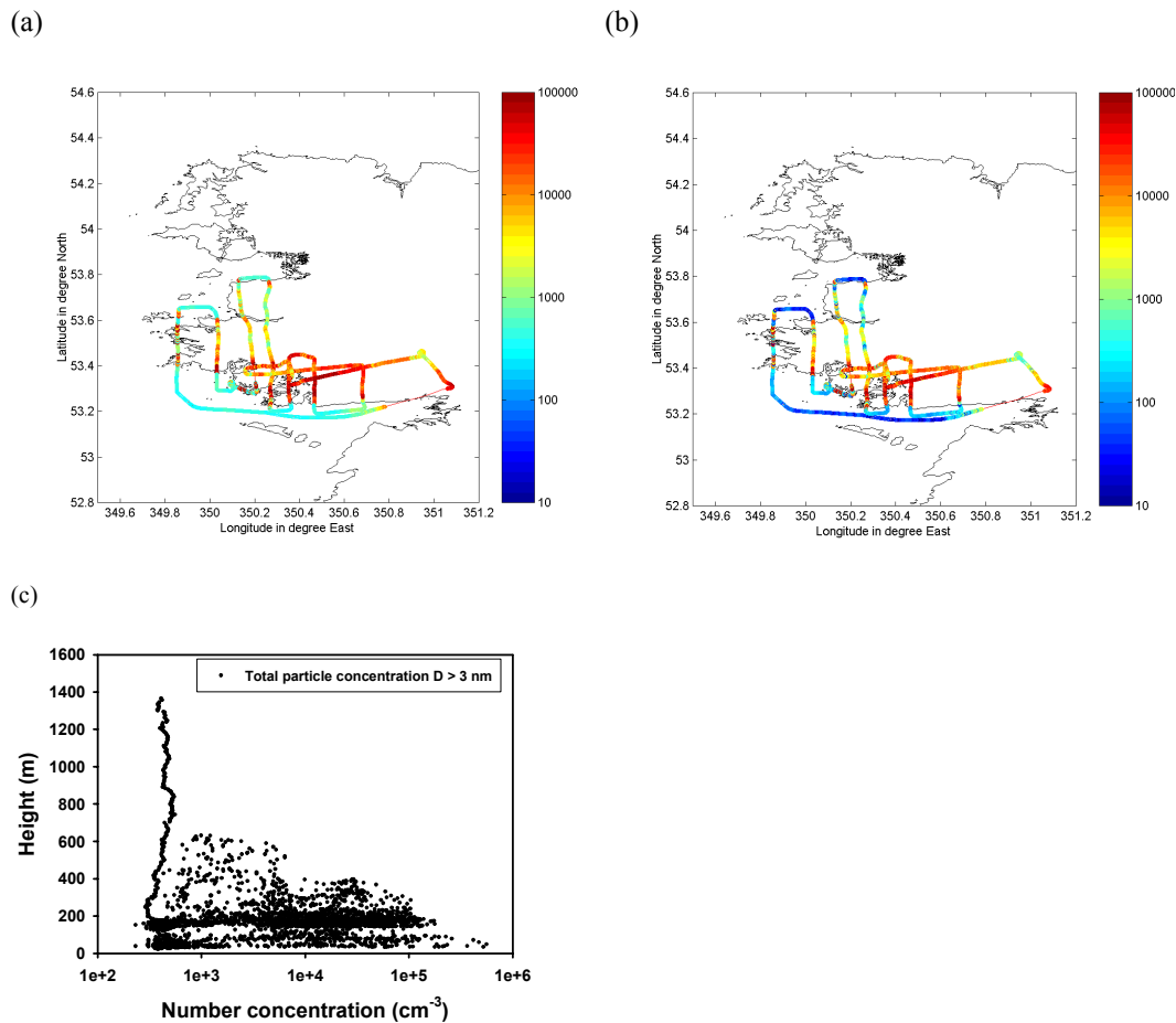
Fig. 3. (a) Total particle concentration for d > 3 nm during flight on 27 May 2002. (b) Same as (a) except for total particle concentration at sizes 3 < d < 10 nm, and (c) Scatter plot of total particle number concentration ( D > 3 nm) versus height from the mapping flight on 27 May 2002. Concentrations units are particles \text{cm}^{-3} . 8119
