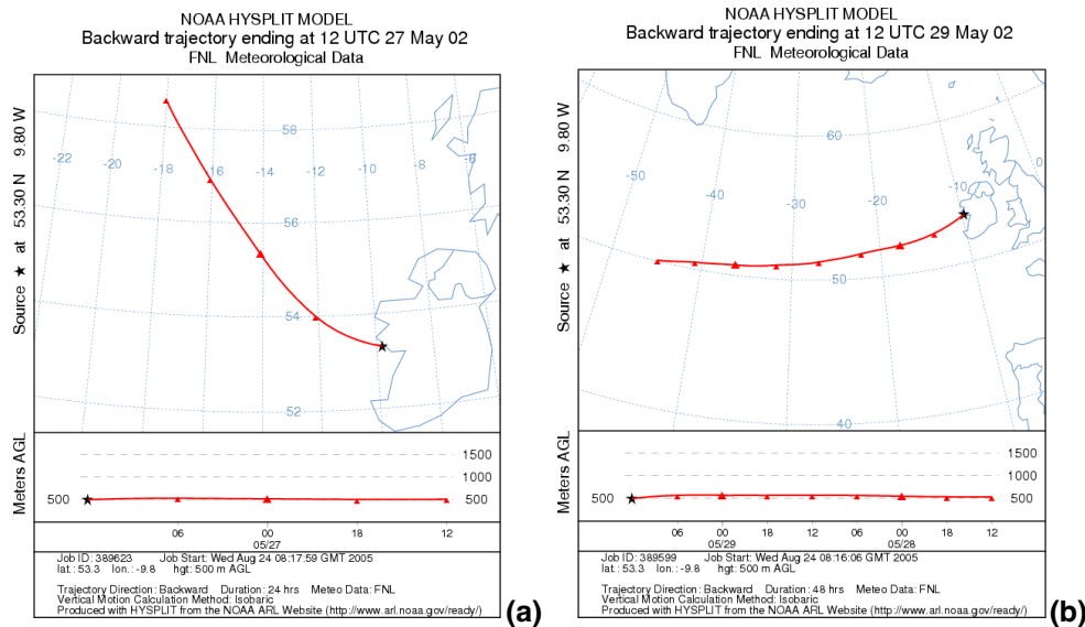
Fig. 2. Air mass back trajectories arriving at Mace Head for (a) on 27 May 2002 and (b) on 29 May 2002.
