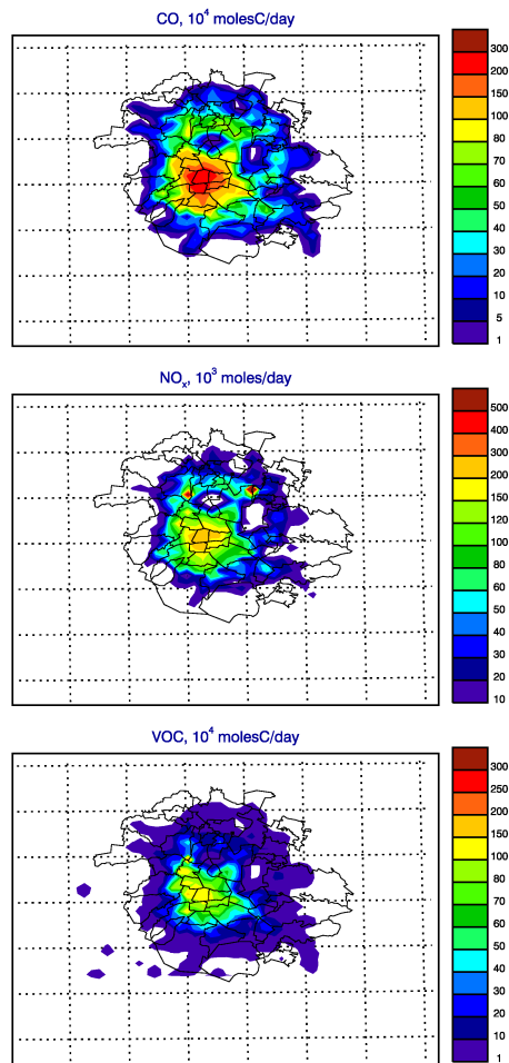
Fig. 2. Spatial distribution of CO, NO x and VOC emissions for a normal weekday in the initial estimates from the 2002 official emission inventory.
