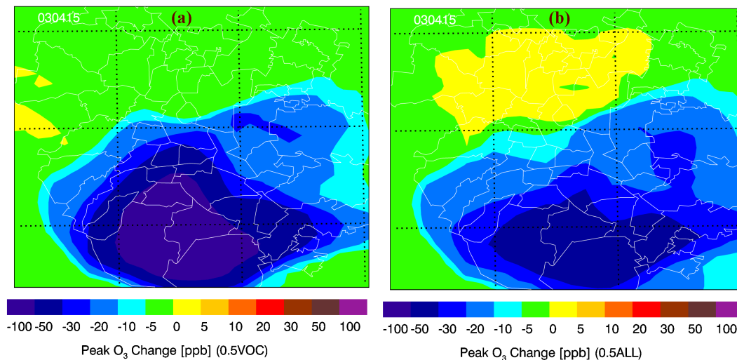
Fig. 14. Change of peak O 3 in the model bottom layer on 15 April 2003 due to a 50% reduction in the emissions of (a) VOCs only and (b) NO x and VOCs both.
