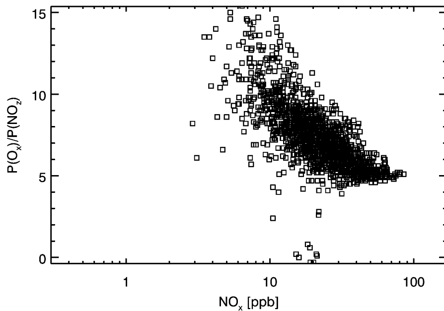
Fig. 9. Simulated relationship between ozone production efficiency ( P(O_x)/P(NO_z) ) and NO_x at 12:00–17:00 CDT during 13–15 April 2003 in the model bottom layer over the urban region.
