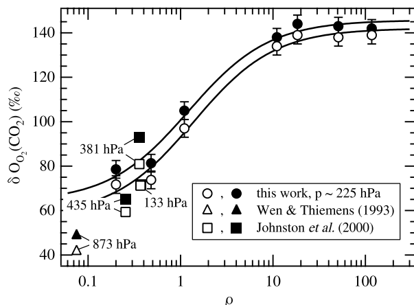
Fig. 3. Dependence on the mixing ratio \rho = [\text{O}_2]/[\text{CO}_2] . 17 O and 18 O containing CO 2 is represented by open and solid symbols, respectively. Data are at constant pressure p \sim 225 hPa (see Table 1) and error bars denote 2\sigma uncertainties. Comparison with data from the literature is indicated and the particular pressure conditions of these measurements are noted. Solid lines describe the weighted average of two a-priori unknown isotopic sources with relative weights 1/(1+\rho/\rho_0) and (\rho/\rho_0)/(1+\rho/\rho_0) , according to Eq. (2).
