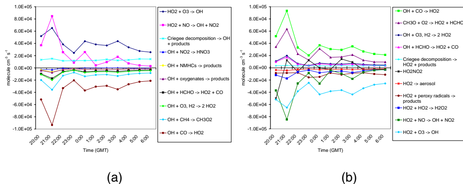
Fig. 5. Rates of production and destruction of OH (a) and HO 2 (b) during the night of 31 August–1 September.
