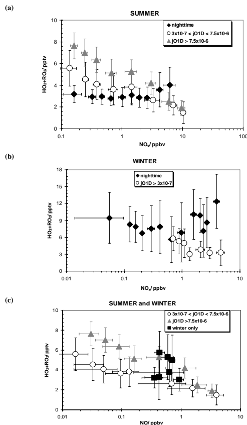
Fig. 8. (a) and (b): Hourly peroxy radical concentration vs. binned hourly \text{NO}_x concentrations for daylight and nighttime conditions for summer (high and low j(\text{O}^1\text{D}) and nighttime) and winter ( j(\text{O}^1\text{D}) > 3 \times 10^{-7} \text{ s}^{-1} (daytime) and nighttime); (c) Hourly peroxy radical concentrations vs. binned hourly \text{NO} concentrations are also plotted for both winter and summer daylight hours.
