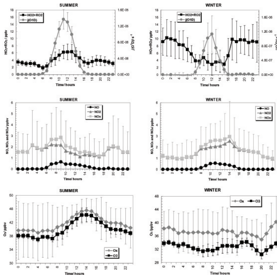
Fig. 7. Campaign hourly averages showing diurnal cycles of peroxy radicals and j(\text{O}^1\text{D}) (note factor of 10 difference in scale between winter and summer), NO x (and NO and NO 2 ) and O 3 and O x (NO 2 +O 3 ) for summer and winter. The bars represent 1σ standard deviation.
