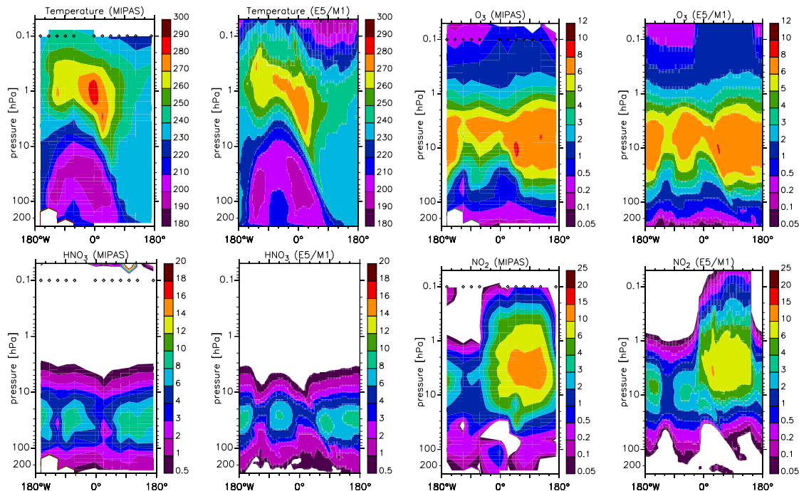
Fig. 9. MIPAS observations and model simulations (E5/M1, S1) of temperature (K), ozone ( \mu\text{mol/mol} ), \text{HNO}_3 ( \text{nmol/mol} ), and \text{NO}_2 ( \text{nmol/mol} ) for 22 September 2002, at 63^\circ\text{S} . Between about 30^\circ\text{W} and 150^\circ\text{E} is night. Diamonds mark longitudes of measurements.
