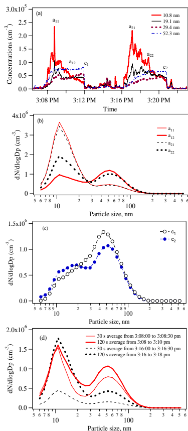
Fig. 5. Ultrafine particle number concentrations and size distributions in Tate Cairn's Tunnel, 7 October 2004. Concentrations of (a) 10.8, 19.1, 29.4 and 52.3 nm particles, (b) Size distributions at a_{11} , a_{12} , a_{21} and a_{22} , (c) Size distribution at c_1 , c_2 , (d) 30 s and 120 s time-averaging spectra. Note: a_{mn} are bi-modal size distributions at \sim 10 nm and \sim 50 nm; c_n are tri-modal size distributions at \sim 10 nm, \sim 20 nm and \sim 50 nm; the subscripts reflects different times.
