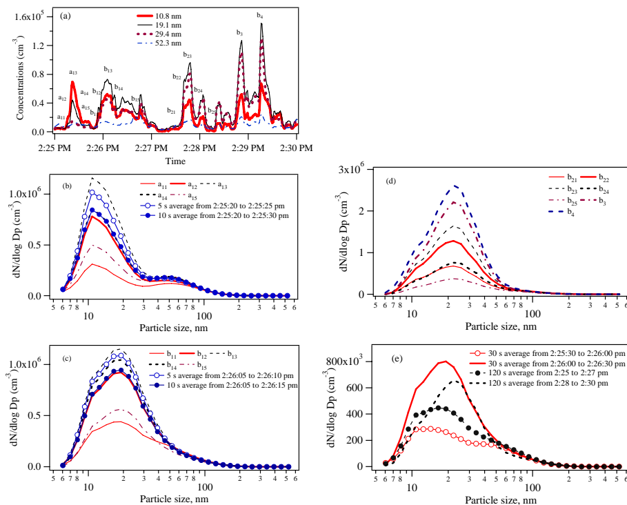
Fig. 1. Light traffic roadside ultrafine particle concentrations and size distributions, 02:30 p.m., 7 October 2004. (a) Concentrations of 10.8, 19.1, 29.4 and 52.3 nm particles, (b) Size distributions and 5 s and 10 s time-averaged spectra at a_{11} – a_{15} , (c) Size distributions and 5 s and 10 s time-averaged spectra at b_{11} – b_{15} , (d) Size distributions at b_{21} – a_{25} , b_{3-4} , (e) 30 s and 120 s time-averaged spectra. Note: a_{1n} are bi-modal size distributions at \sim 10 nm and \sim 50 nm, b_m and b_{mn} are bi-modal size distributions at \sim 10 nm and \sim 20 nm; the subscripts reflect different times.
