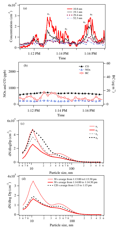
Fig. 4. On road ultrafine particle number concentrations and size distributions, 8 October 2004. (a) Concentrations of 10.8, 19.1, 29.4 and 52.3 nm particles, (b) CO (ppb), NO x (ppb) and BC ( \mu\text{g m}^{-3} ), (c) Size distributions at a_1 , a_2 , a_3 and a_4 , (d) 30 s and 120 s time-averaging spectra. Note: a_n are bi-modal size distributions at \sim 10 nm and \sim 50 nm and the subscripts reflect different times.
