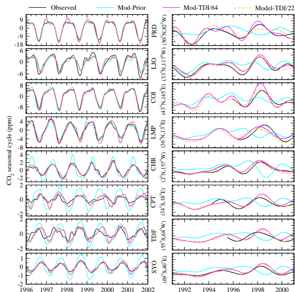
Fig. 5. Timeseries of observed seasonal cycles (left column) and growth rates (right column) at 8 stations worldwide are compared with NIES/FRCGC model simulations using three flux scenarios. The observed curves are shown for the periods with data gaps less than an year. Note that the seasonal cycles and growth rates are shown for different period for better clarity. In addition, the y-axis ranges are different for each panel on left column. The abbreviated station names and locations (latitude, longitude) are given between the two columns (see Table 2 for full names). The CO 2 data are obtained from following organisations for GlobalView analysis; FRD: Meteorological Service of Canada (MSC), LJO: Scripps Institution of Oceanography (SIO), United States, COI: National Institute for Environmental Studies (NIES), Japan, LMP: National Agency for New Technology, Energy, and Environment (ENE), Italy, CHR: NOAA/Global Monitoring Division (GMD), United States, CPT: South African Weather Service (SAWS), TDF: NOAA/Global Monitoring Division (GMD), and SYO: National Institute of Polar Research in cooperation with Tohoku University (NIPR/TU), Japan (see the GLOBALVIEW-CO 2 documentation for further details).
