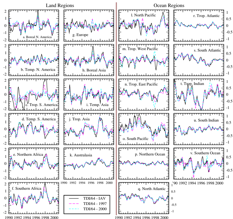
Fig. 4. A comparison of CO 2 flux anomalies for 22 regions of the globe is shown (11 land: two left columns, and 11 ocean: two right columns); fluxes are derived using the 64-region TDI model with varying TTM meteorology. A long-term mean seasonal cycle for each region is subtracted from the TDI model derived monthly fluxes to calculate the anomalies. Five-month running averages are taken to reduce the high frequency variability in fluxes and all values on the y-axis (flux anomaly) are in Pg-C yr -1 . Two common y-axis scales (on the left and on right) are used for the land and ocean fluxes, respectively.
