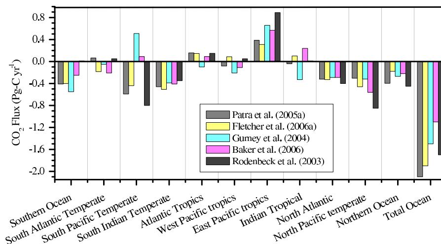
Fig. 3. Comparison of CO 2 flux estimates using an ocean inversion and atmospheric inversions using different modeling frameworks. The regional fluxes of higher resolution inverse models are aggregated to TransCom-3 regions (subcontinental scale). Rödenbeck et al. (2003) fluxes are the average of the inversion cases used in this study (refer to their Fig. 8) and correspond to the 1990s. Gurney et al. (2004) and Baker et al. (2006) fluxes correspond to the periods 1992–1996 and 1991–2000, respectively.
