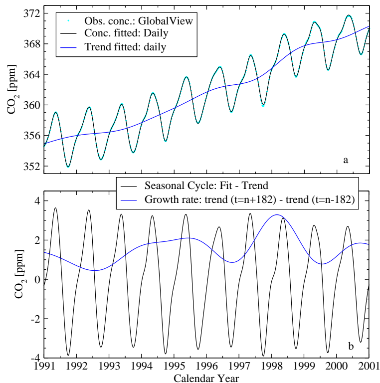
Fig. 2. An example of the extraction of seasonal cycles and growth rates (b) from atmospheric-CO 2 observations (a) at Mauna Loa (19° N, 156° W) is depicted.
