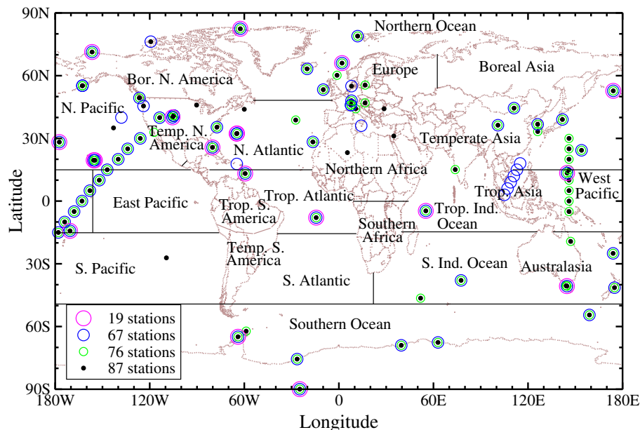
Fig. 1. The atmospheric-CO 2 measurement networks used in this study are shown. These networks are similar to those used in Bousquet et al. (2000): 67 stations, TransCom (Gurney et al., 2004): 76 stations, Rödenbeck et al. (2003b): 19 stations, and Patra et al. (2005a): 87 stations. The 22 TDI model regions are also shown; the 64-region TDI model has 4 divisions for the land regions (except for Tropical Asia) and the ocean regions are divided into two along the longitude (see Patra et al., 2005a, b, for further details).
