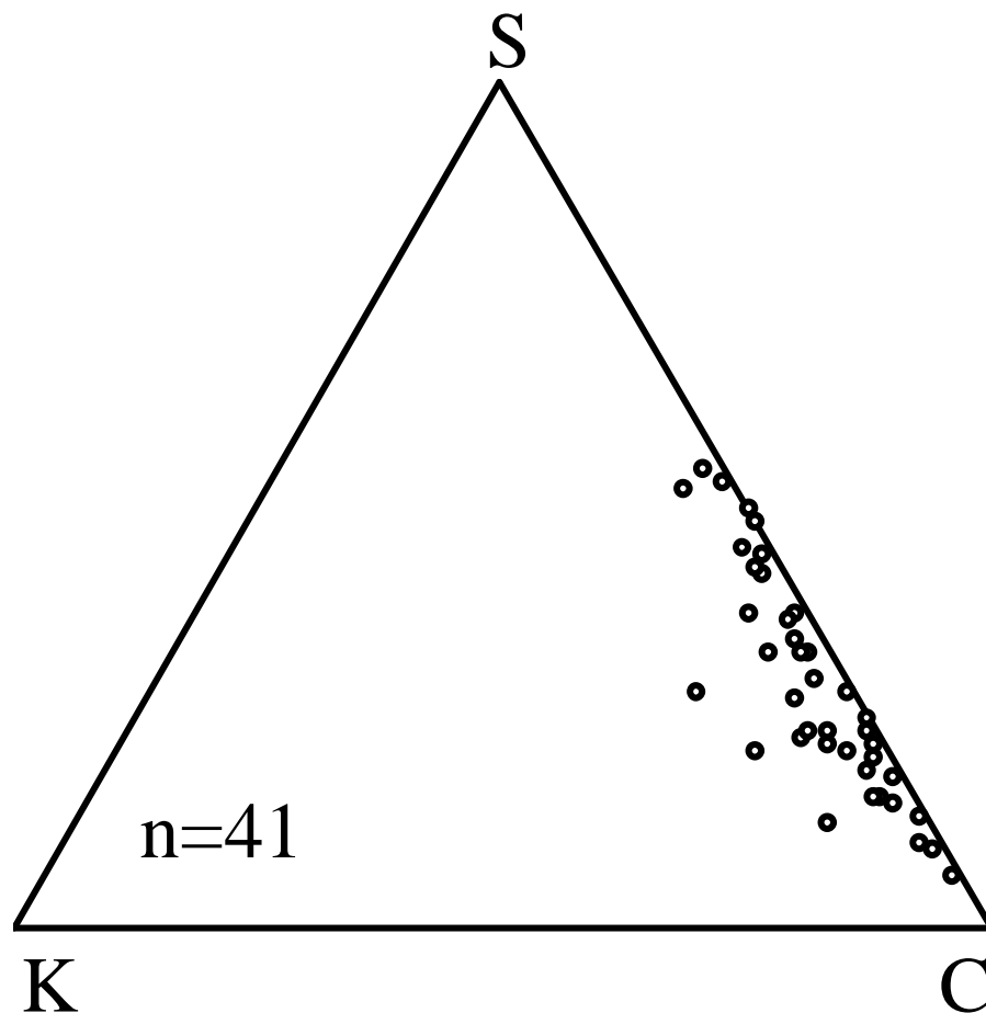
Fig. 7. Ternary diagram of C-S-K ratios for particles in “carbon/sulphate mixture with dark inclusion(s)” group from all PM_{0.2-1} samples.
