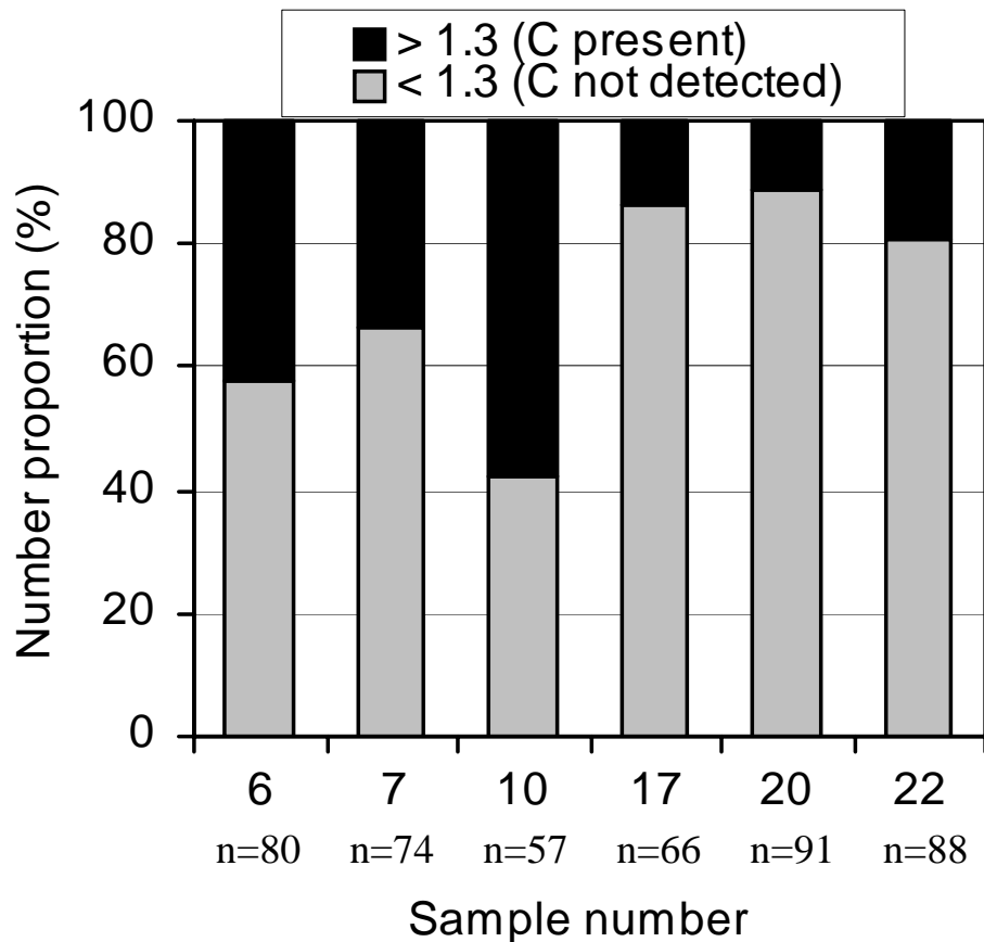
Fig. 8. Relative proportion of ammonium sulphate particles with detectable carbon (with total C peak to background C peak ratio >1.3 as indicator) and without detectable carbon (the same ratio <1.3) from PM 0.2-1 samples.
