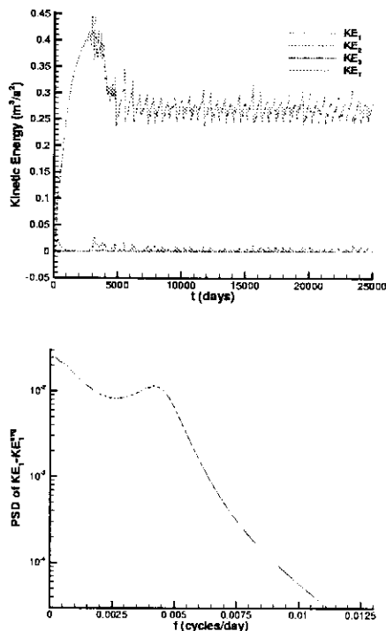
Fig. 22. Spatially-averaged kinetic energy and the corresponding power spectrum for the upper layer when \tau_0 = 0.170 dyn/cm 2 . The spectrum shows the same characteristics as in the case shown in Fig. 19.
