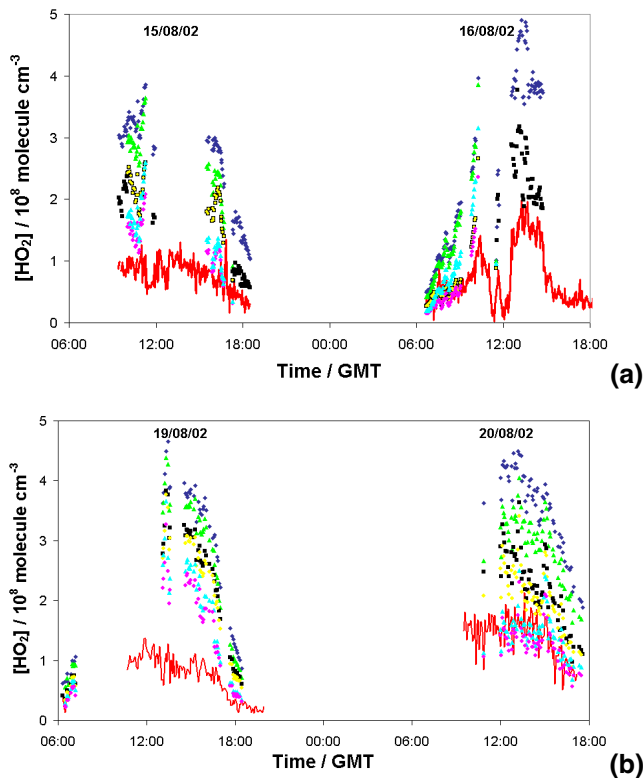
Fig. 8. Diurnal profiles of measured HO 2 (red line), and steady-state calculated HO 2 derived using Eq. (5) (navy blue diamonds) and several modifications which also include: loss by reaction of HO 2 with measured IO (green triangles), loss by reaction of HO 2 with measured IO \times 10 (light blue triangles), uptake of HO 2 onto aerosol (black squares), both loss of HO 2 by reaction with IO and by uptake onto aerosol (yellow circles with or without black border) and both loss of HO 2 by reaction with IO \times 10 and uptake onto aerosols (pink circles). The data shown are from (a) 15–16 August (b) and 19–20 August. It was not possible to calculate HO 2 between 11:57 and 15:26 GMT on the 15 August as O 3 data adjacent to the FAGE instrument were not available.
