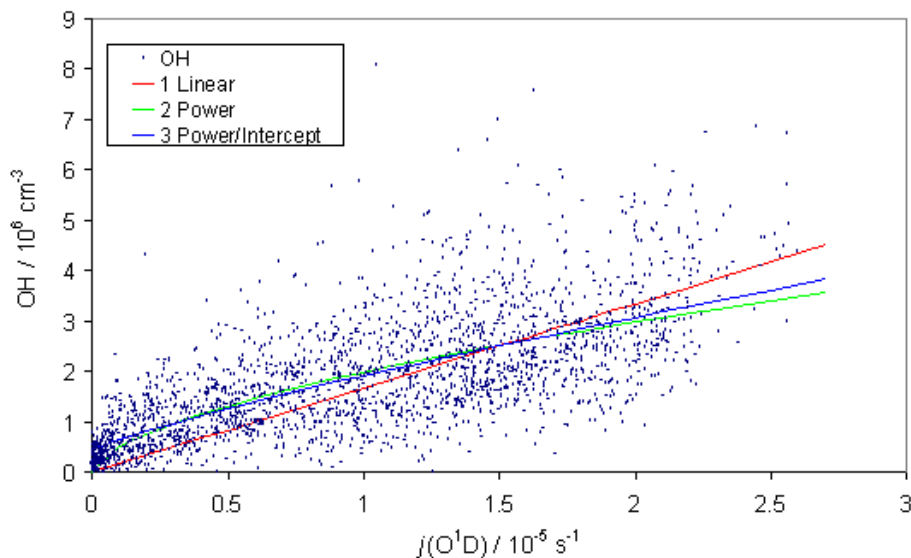
Fig. 5. Measured OH data from the NAMBLEX campaign plotted against j(\text{O}^1\text{D}) (measured by a spectral radiometer), together with fits to three versions of Eq. (10): (1) Linear (red line), (2) Power (green line) and (3) Power with intercept (blue line). See text for details.
