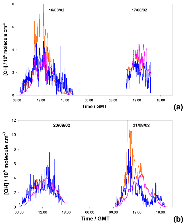
Fig. 6. Diurnal profiles of measured OH (blue line), OH calculated using the simple steady state expression Eq. (4), which includes primary production from O 3 photolysis; and loss by reaction of CO and CH 4 only (pink line), and OH calculated by a more complex steady state expression (Eq. (11)), which also includes HO 2 +NO and HO 2 +O 3 as OH sources, and also OH loss by reaction with o -VOCs (orange line) for representative 2-day periods: (a) 16–17 August (b) 20–21 August.
