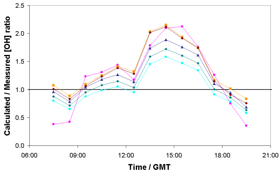
Fig. 7. Campaign averaged diurnal of the hourly average calculated/measured [OH] ratio for Eq. (4) (pink circles), Eq. (11) (orange squares), Eq. (11) including loss of OH to NO 2 (brown diamonds), Eq. (11) including loss of OH to NO 2 and HCHO (navy blue triangles), Eq. (12) which includes all of the above and also reaction with non-methane hydrocarbons (light blue circles), and Eq. (12) but excluding isoprene and DMS (green diamonds). The graph is constructed from 522×200 s averaged data points taken on 8 days between 10 and 21 August when all co-reactant data were available. Uncertainties are omitted for clarity. The mean calculated/measured OH ratios for all calculations are summarised in Table 3.
