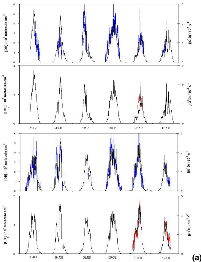
Fig. 2. Time-series of OH (blue) and HO 2 (red) concentrations during NAMBLEX. Each point represents a 5 min collection period comprising 10 adjacent 20 s online data points with a consecutive background period consisting of 5 adjacent 20 s data points. 5 min averaged j -(O 1 D) (black) as measured by a spectral radiometer, are also shown.
