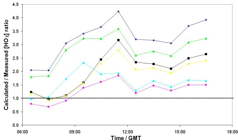
Fig. 9. Campaign average of the hourly averaged calculated/measured [HO 2 ] ratio using Eq. (5) (navy blue diamonds) and several modifications which also include: loss by reaction of HO 2 with measured IO (green triangles), loss by reaction of HO 2 with measured IO×10 (light blue triangles), uptake of HO 2 onto aerosol (black squares), both loss of HO 2 by reaction with IO and by uptake onto aerosol (yellow circles) and both loss of HO 2 by reaction with IO×10 and uptake onto aerosol (pink circles). The graph is constructed from 281×200 s averaged data points on 6 days (13, 15–16, 19–21 August) when all co-reactant data were available. Uncertainties are omitted for clarity. The mean calculated/measured HO 2 ratios for all calculations can be found in Table 4.
