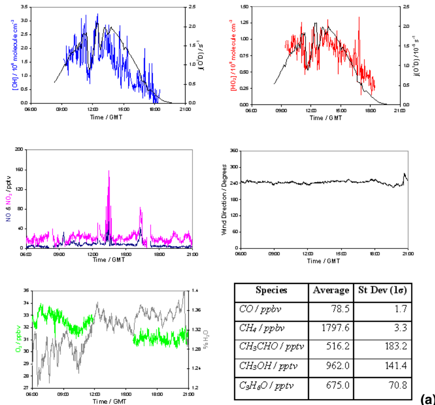
Fig. 4. Time-series and a table of other relevant information are shown for the four case study days described in Sect. 4.2 of the text; (a) 15 August, (b) 16 August, (c) 18 August and (d) 21 August. The top 2 panels show 200 s averaged OH (blue) and HO 2 (red) (recorded in a 5 min cycle which includes background measurements) with 5 min average j –(O 1 D) (black). The middle panels show NO (navy blue) and NO 2 (pink), and wind direction (black). The bottom panels show O 3 (green) and H 2 O (grey), and a table of the daily average CO, CH 4 , acetaldehyde, methanol and acetone concentrations together with their respective 1\sigma variability.
