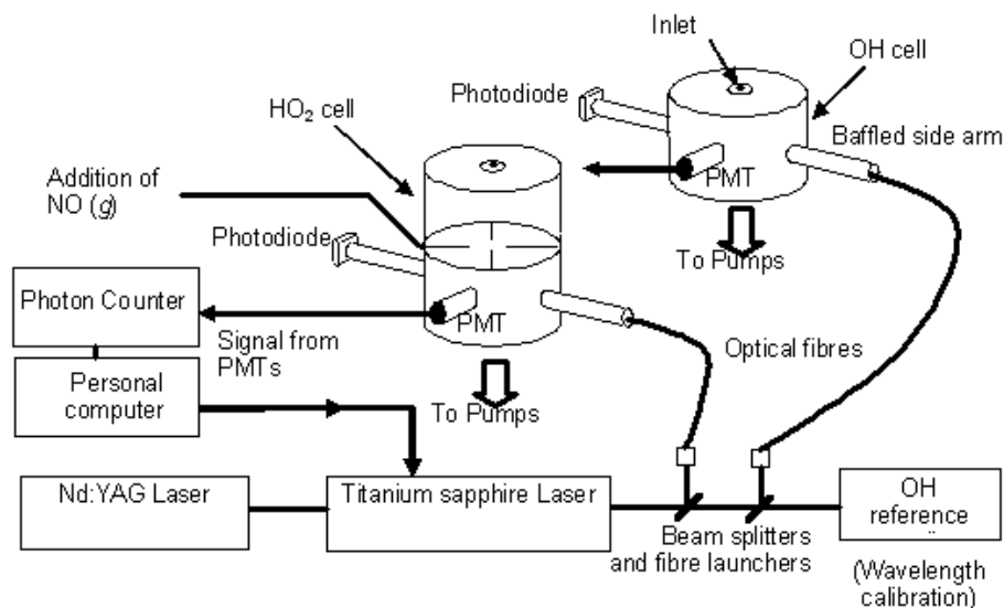
Fig. 1. A schematic of the FAGE instrument as deployed during the NAMBLEX campaign.
