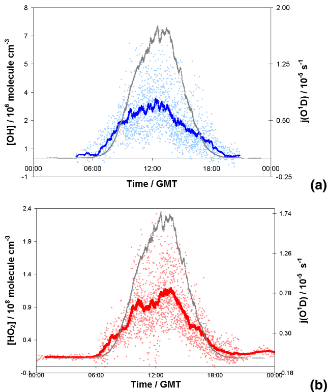
Fig. 3. (a) Diurnal profile of all OH data (200 s averages) for the campaign (light blue circles), together with a 40 point running mean of the OH data, (dark blue lines) and a campaign averaged j(O^1D) (grey line). (b) Diurnal profile of all HO 2 data (200 s averages) for the campaign (pink diamonds), together with a 40 point running mean (red line) and a campaign averaged j(O^1D) (grey line).
