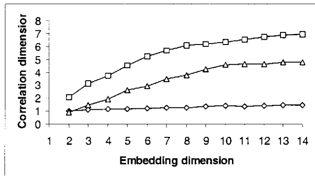
Fig. 8 Correlation dimension versus embedding dimension for the Javakheti enlarged area inter-event time interval sequences: a) 10 km enlargement. b) 20 km enlargement. Lower curves: original sequences, middle and upper curves: Gaussian scaled random phases and phase randomized inter-event time interval surrogates, respectively.
