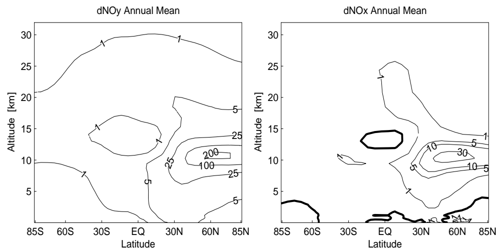
Fig. 4. Annually averaged changes in zonal-mean \text{NO}_y (left) and \text{NO}_x (right) due to aircraft emissions in the TRADEOFF reference case, i.e. 'yy-00' (units: pptv). Contours at -1, 0, 1, 5, 25, 100, 200 for \text{NO}_y , and -1, 0, 1, 5, 10, 30 for \text{NO}_x .
