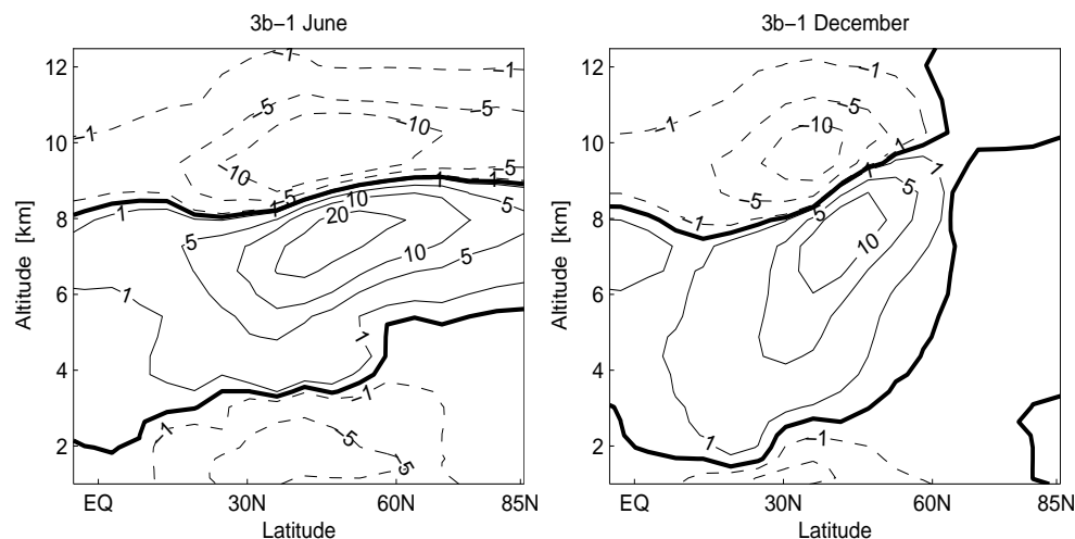
Fig. 14. Change in net chemical ozone production ( 10^3 \text{ molecules cm}^{-3} \text{ s}^{-1} ) due to a 1830 m reduction in flight altitude, taking into account changes in fuel consumption, i.e. '3b minus 1' in June (left) and December (right). Contours at -20, -10, -5, -1, 0, 1, 5, 10, and 20.
