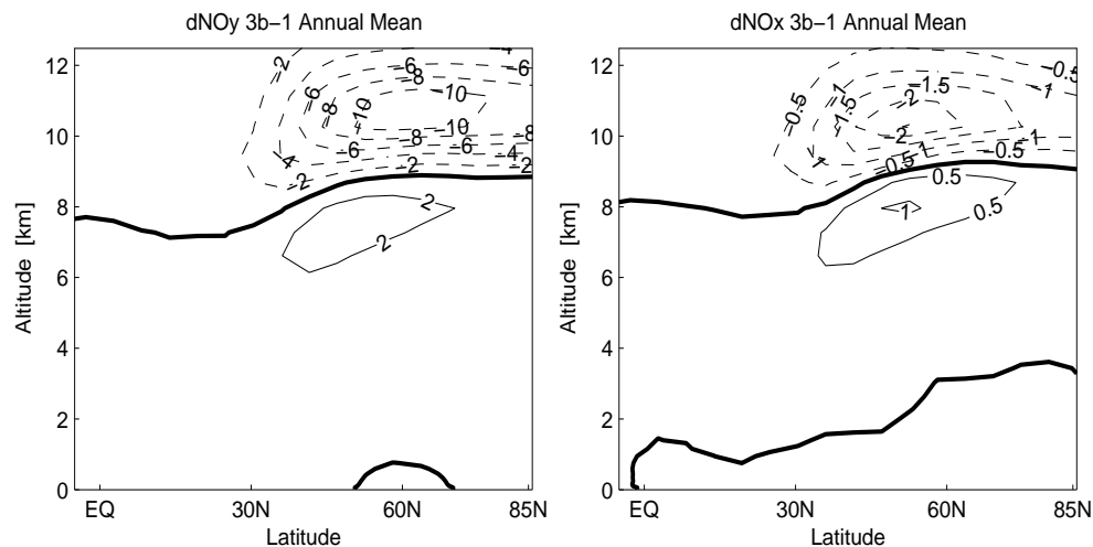
Fig. 13. Annual-mean changes in concentrations of NO y (top left, 10^8 molecules \text{cm}^{-3} ) and NO x (top right, 10^8 molecules \text{cm}^{-3} ) in the Northern Hemisphere due to a 1830 m reduction in flight altitude taking into account changes in fuel consumption, i.e. ‘3b minus 1’. Contours at -12, -10, -8, -6, -4, -2, 0, 2 for NO y and -2.5, -2, -1.5, -1, -0.5, 0, 0.5, 1 for NO x .
