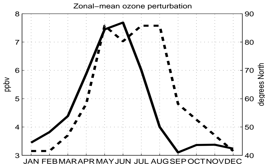
Fig. 7. Maximum increase in monthly averaged zonal-mean ozone due to aircraft in the TRADE-OFF reference case as a function of season, i.e. 'yy minus 00'. Solid line: magnitude of the maximum (ppbv, left axis), dashed line: latitude at which the maximum increase occurs (degrees North, right axis).
