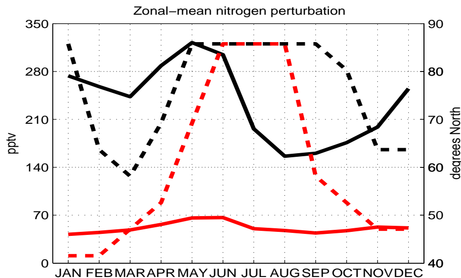
Fig. 5. Maximum increase in monthly averaged zonal-mean \text{NO}_y (black) and \text{NO}_x (red) due to aircraft in the TRADEOFF reference case as a function of season, i.e. 'yy minus 00'. Solid lines: magnitude of the maximum (pptv, left axis), dashed lines: latitude at which the maximum increases occur (degrees North, right axis).
