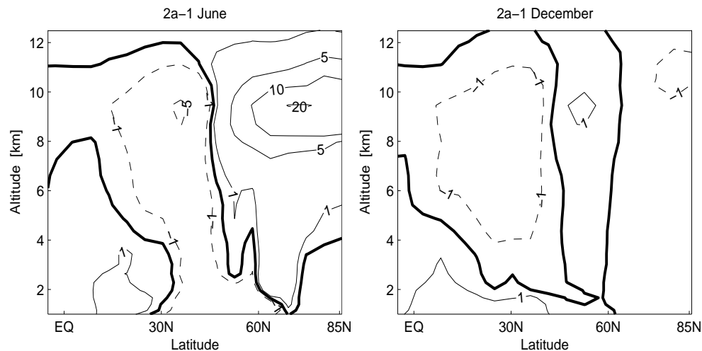
Fig. 9. Change in net chemical ozone production ( 10^3 molecules \text{cm}^{-3} \text{s}^{-1} ) due polar routes replacing conventional routes, i.e. ‘2a minus 1’ in June (left) and December (right). Contours at -5, 1, 0, 1, 5, 10, and 20 .
