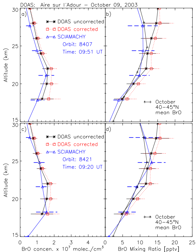
Fig. 6. Same as Fig. 5 but for a comparison with the DOAS balloon flight on 9 October 2003 from Aire sur l'Adoure (43.7° N, balloon SZA=72.9° (p.m.)). Panels (a) and (b) show a backward trajectory match, while panels (c) and (d) show a forward trajectory match. See text for details on the trajectory matches.
