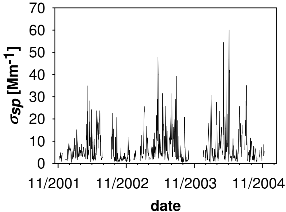
Fig. 2. Time-series of \sigma_{sp} at 550 nm.
