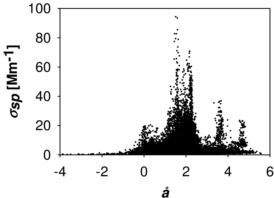
Fig. 7. Relation between \sigma_{sp} at 550 nm and \hat{a} .
